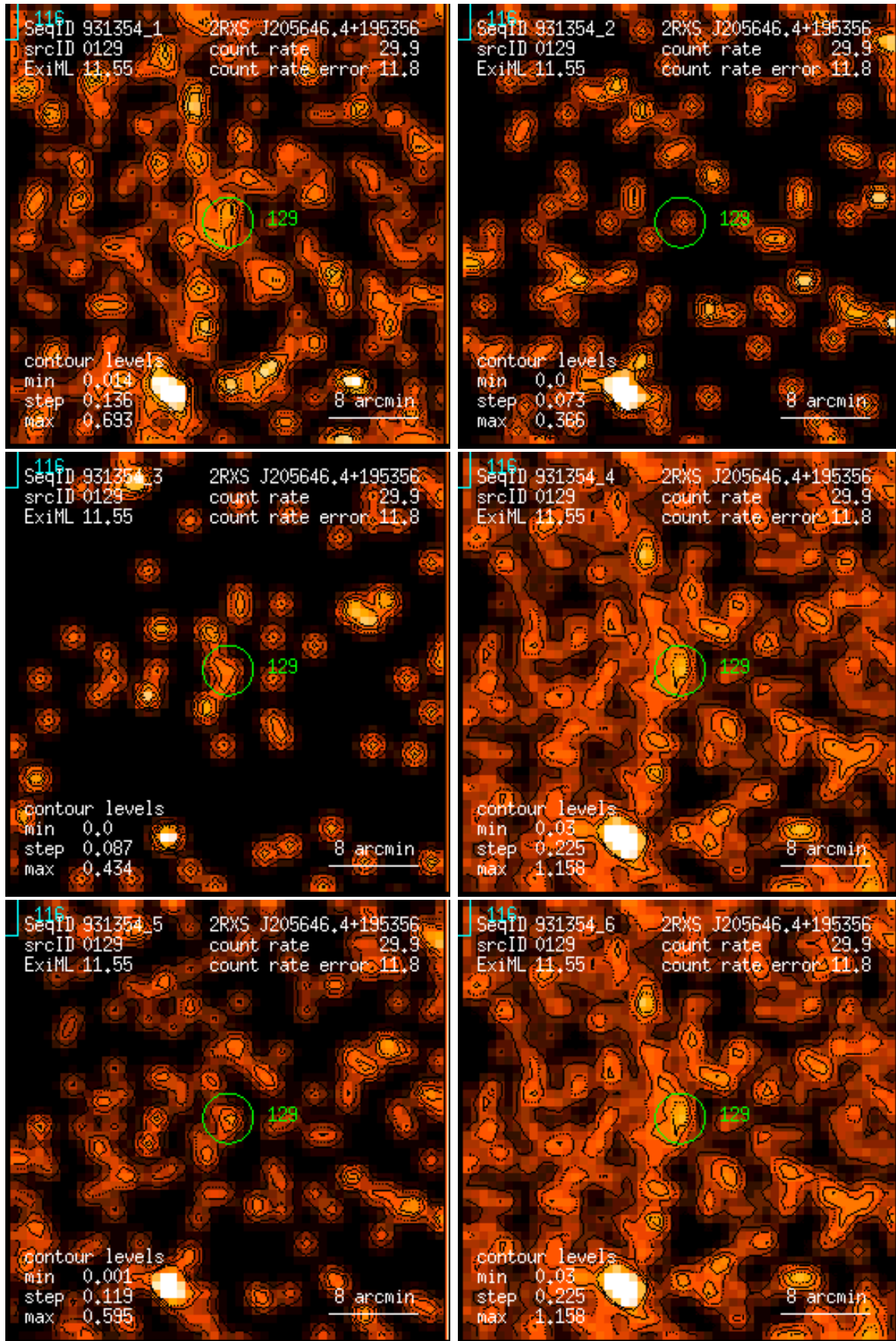
Figure 129: RASS 931354: detection 0129: band rate images, Gaussian filter: (1) PSPC channels 11 – 41, (2) 52 – 90, (3) 91 – 201, (4) 11 – 235, (5) 52 – 201, (6) 11 – 201. Broad band rates in counts/ks. Band rate contour levels in counts/ks/arcmin 2 .
