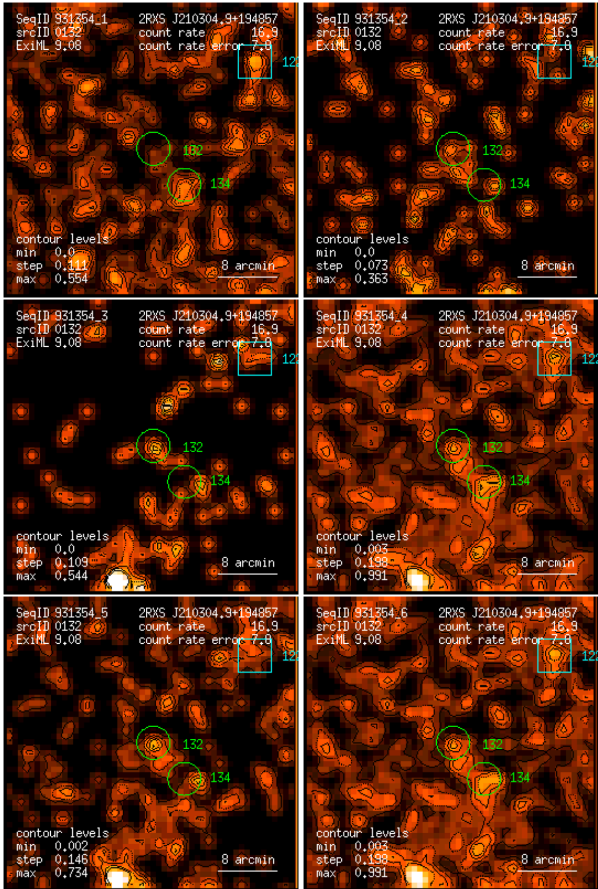
Figure 132: RASS 931354: detection 0132: band rate images, Gaussian filter: (1) PSPC channels 11 – 41, (2) 52 – 90, (3) 91 – 201, (4) 11 – 235, (5) 52 – 201, (6) 11 – 201. Broad band rates in counts/ks. Band rate contour levels in counts/ks/arcmin 2 .
