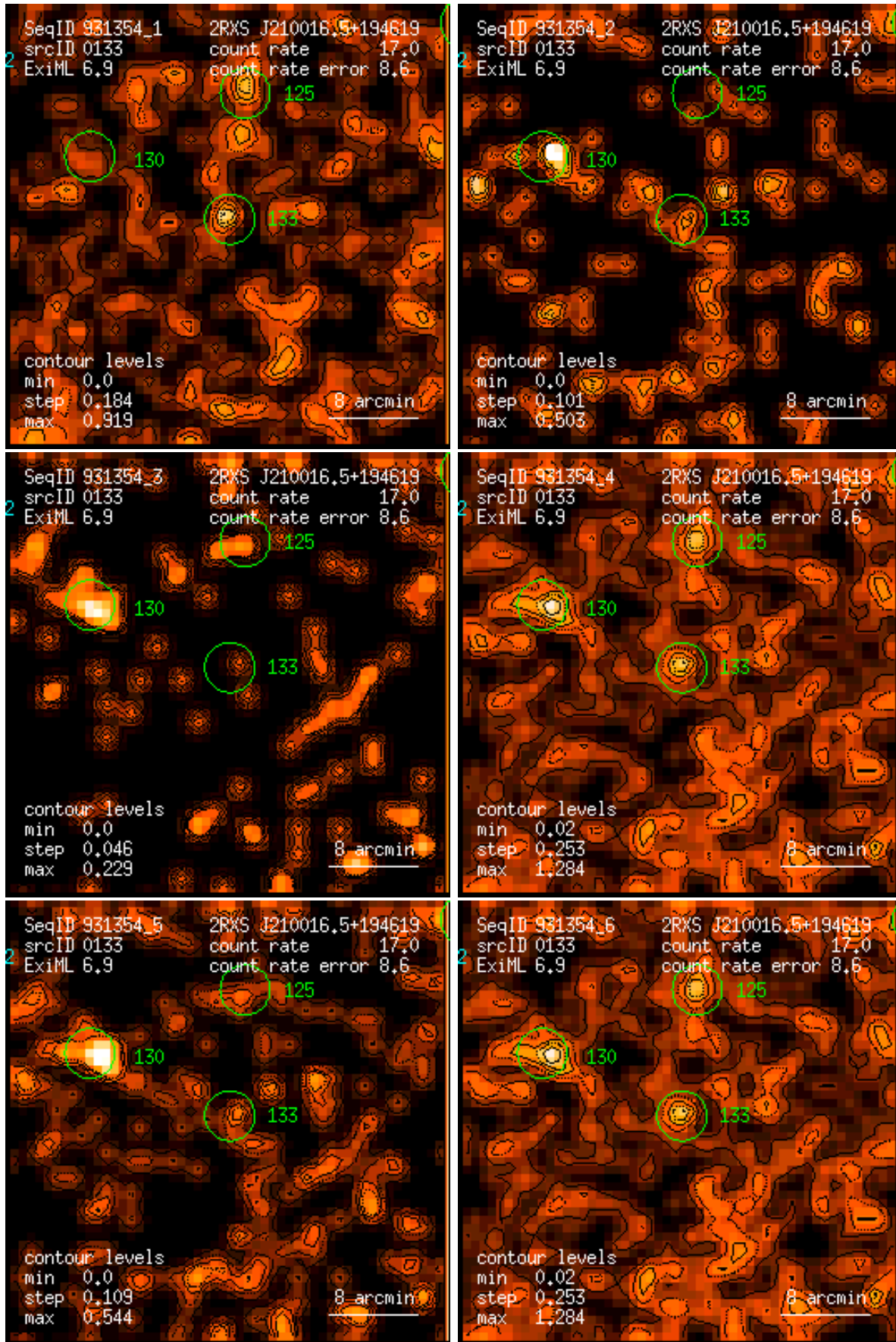
Figure 133: RASS 931354: detection 0133: band rate images, Gaussian filter: (1) PSPC channels 11 – 41, (2) 52 – 90, (3) 91 – 201, (4) 11 – 235, (5) 52 – 201, (6) 11 – 201. Broad band rates in counts/ks. Band rate contour levels in counts/ks/arcmin 2 .
