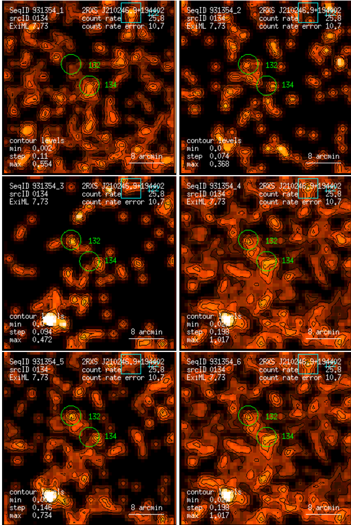
Figure 134: RASS 931354: detection 0134: band rate images, Gaussian filter: (1) PSPC channels 11 – 41, (2) 52 – 90, (3) 91 – 201, (4) 11 – 235, (5) 52 – 201, (6) 11 – 201. Broad band rates in counts/ks. Band rate contour levels in counts/ks/arcmin 2 .
