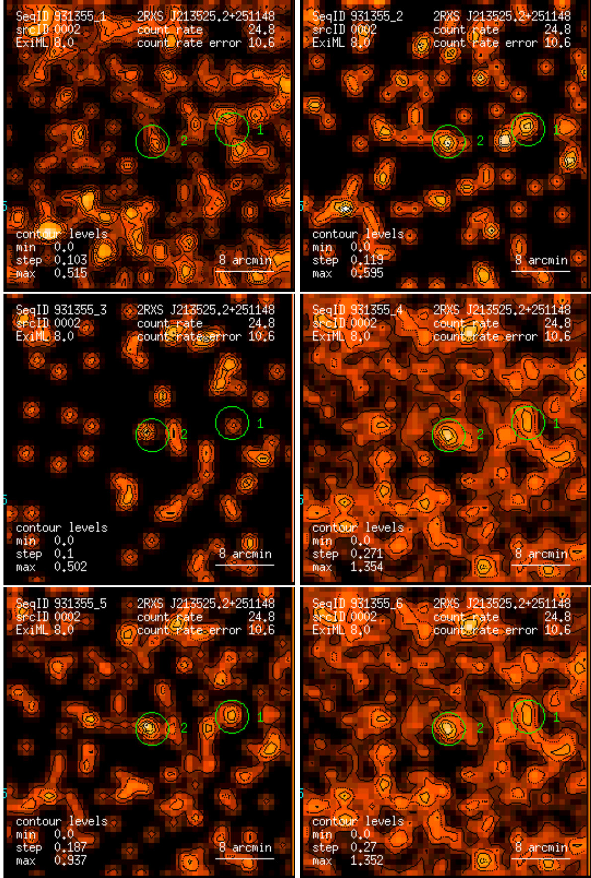
Figure 2: RASS 931355: detection 0002: band rate images, Gaussian filter: (1) PSPC channels 11 – 41, (2) 52 – 90, (3) 91 – 201, (4) 11 – 235, (5) 52 – 201, (6) 11 – 201. Broad band rates in counts/ks. Band rate contour levels in counts/ks/arcmin 2 .
