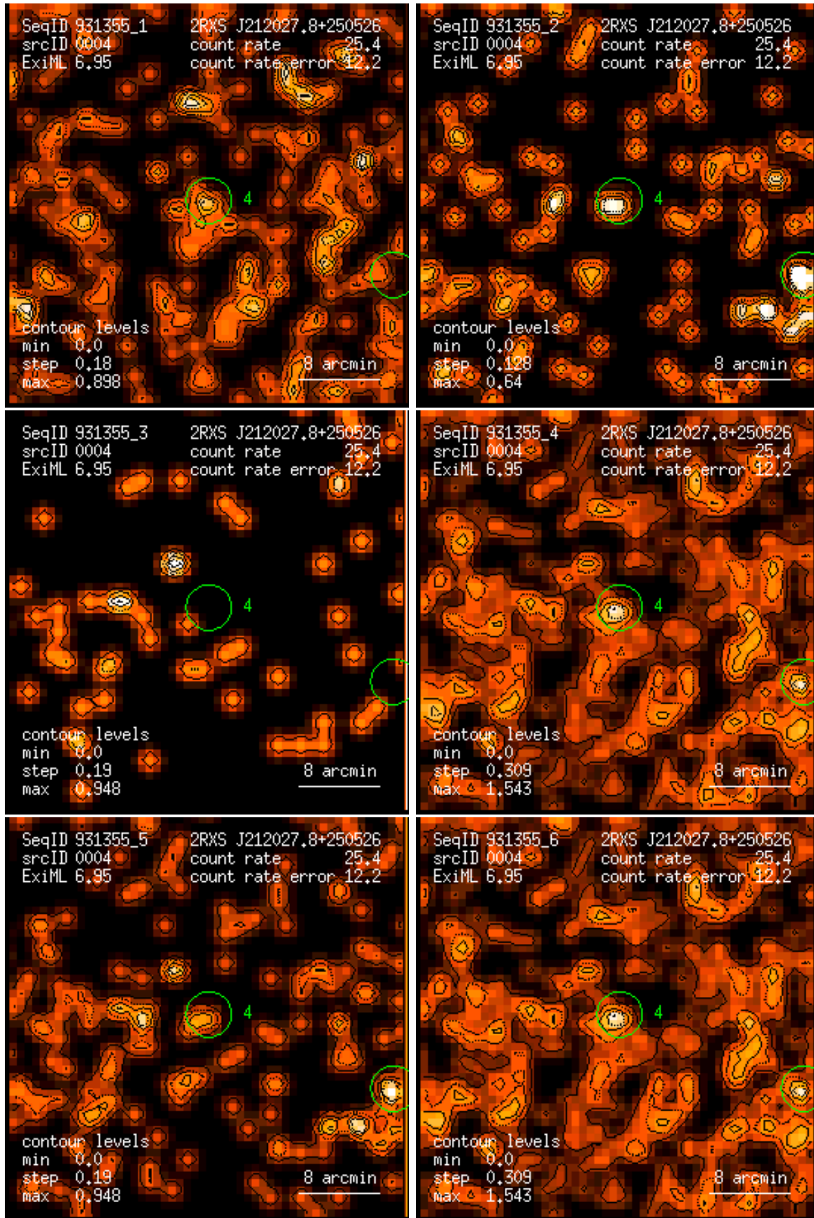
Figure 4: RASS 931355: detection 0004: band rate images, Gaussian filter: (1) PSPC channels 11 – 41, (2) 52 – 90, (3) 91 – 201, (4) 11 – 235, (5) 52 – 201, (6) 11 – 201. Broad band rates in counts/ks. Band rate contour levels in counts/ks/arcmin 2 .
