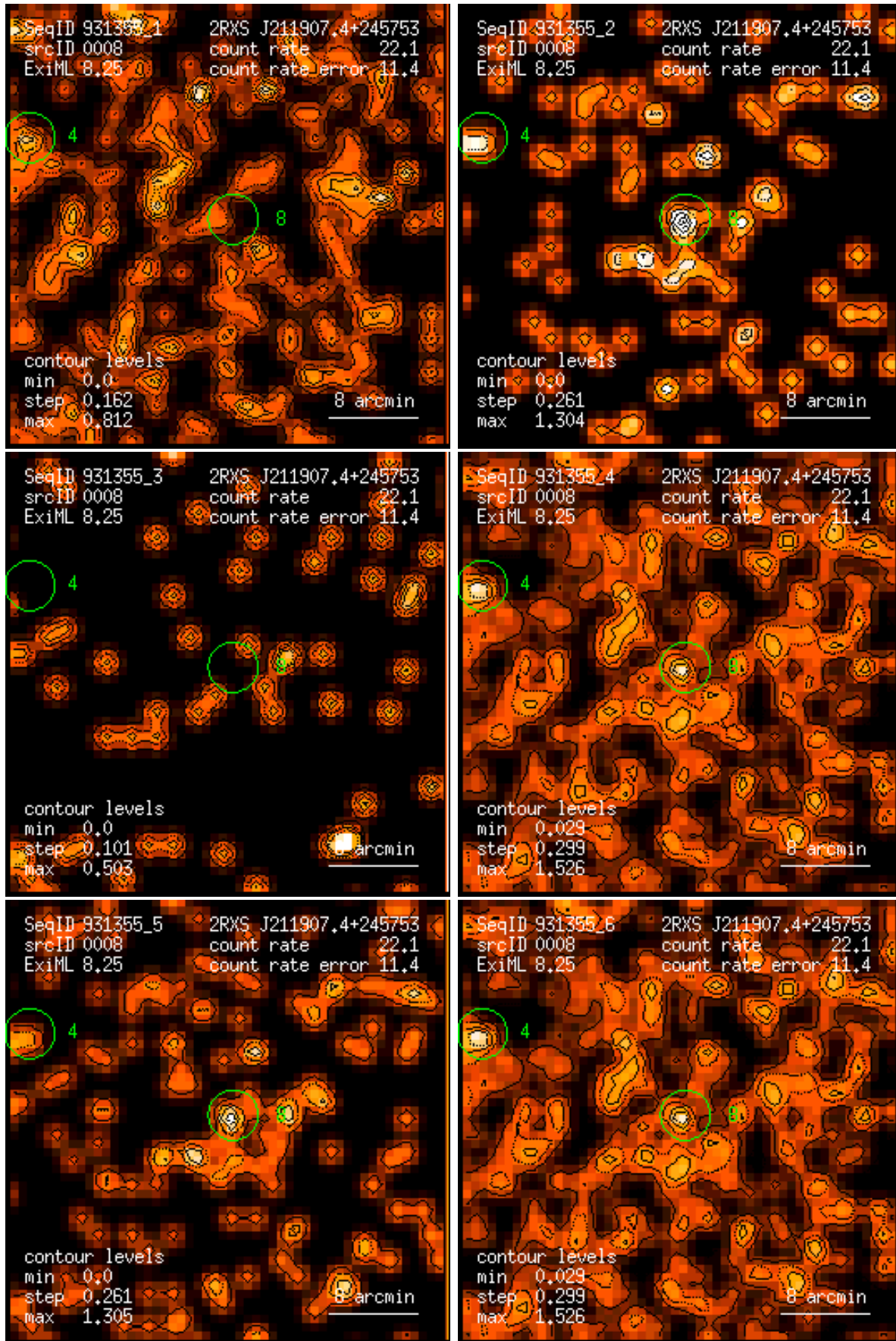
Figure 8: RASS 931355: detection 0008: band rate images, Gaussian filter: (1) PSPC channels 11 – 41, (2) 52 – 90, (3) 91 – 201, (4) 11 – 235, (5) 52 – 201, (6) 11 – 201. Broad band rates in counts/ks. Band rate contour levels in counts/ks/arcmin 2 .
