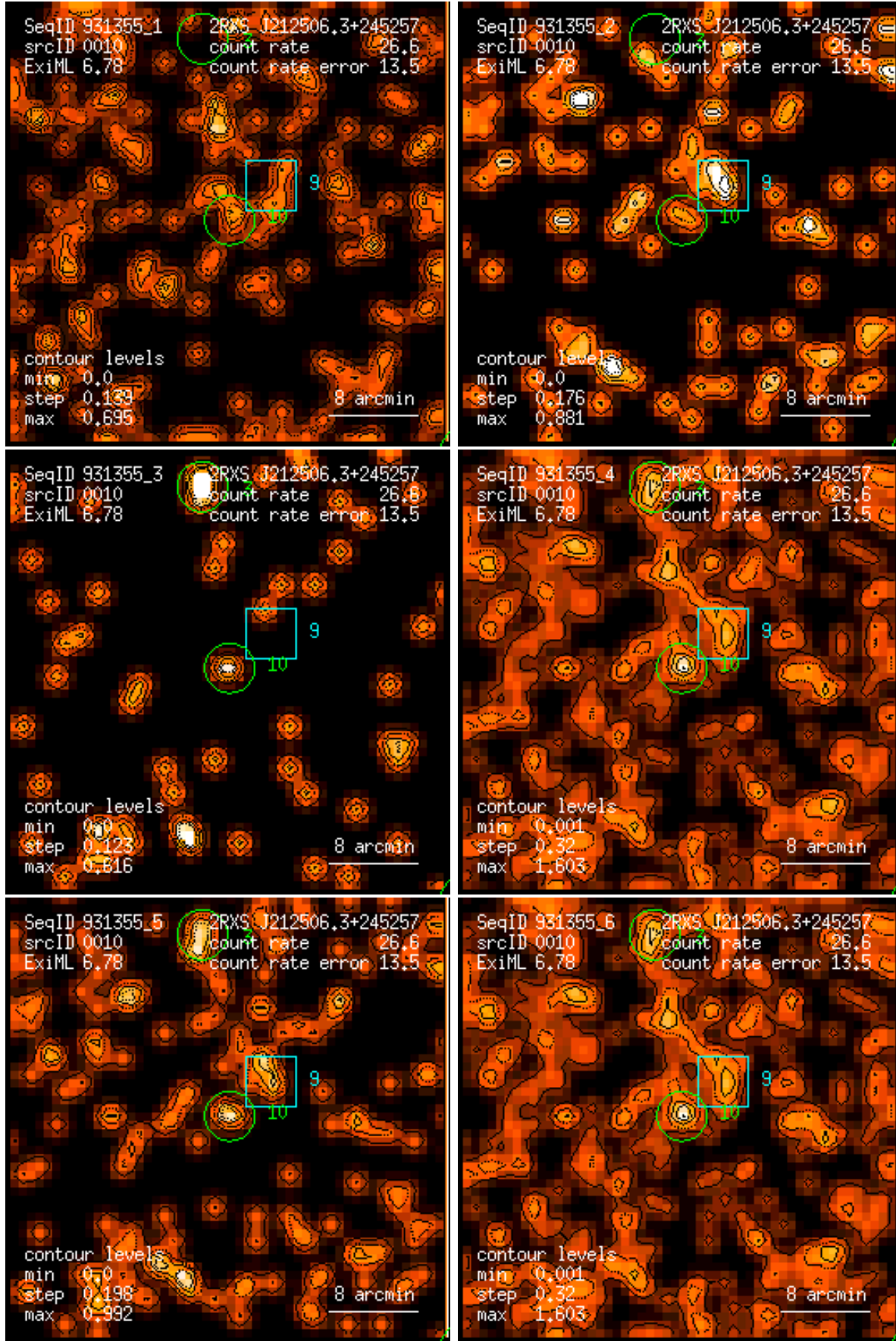
Figure 10: RASS 931355: detection 0010: band rate images, Gaussian filter: (1) PSPC channels 11 – 41, (2) 52 – 90, (3) 91 – 201, (4) 11 – 235, (5) 52 – 201, (6) 11 – 201. Broad band rates in counts/ks. Band rate contour levels in counts/ks/arcmin 2 .
