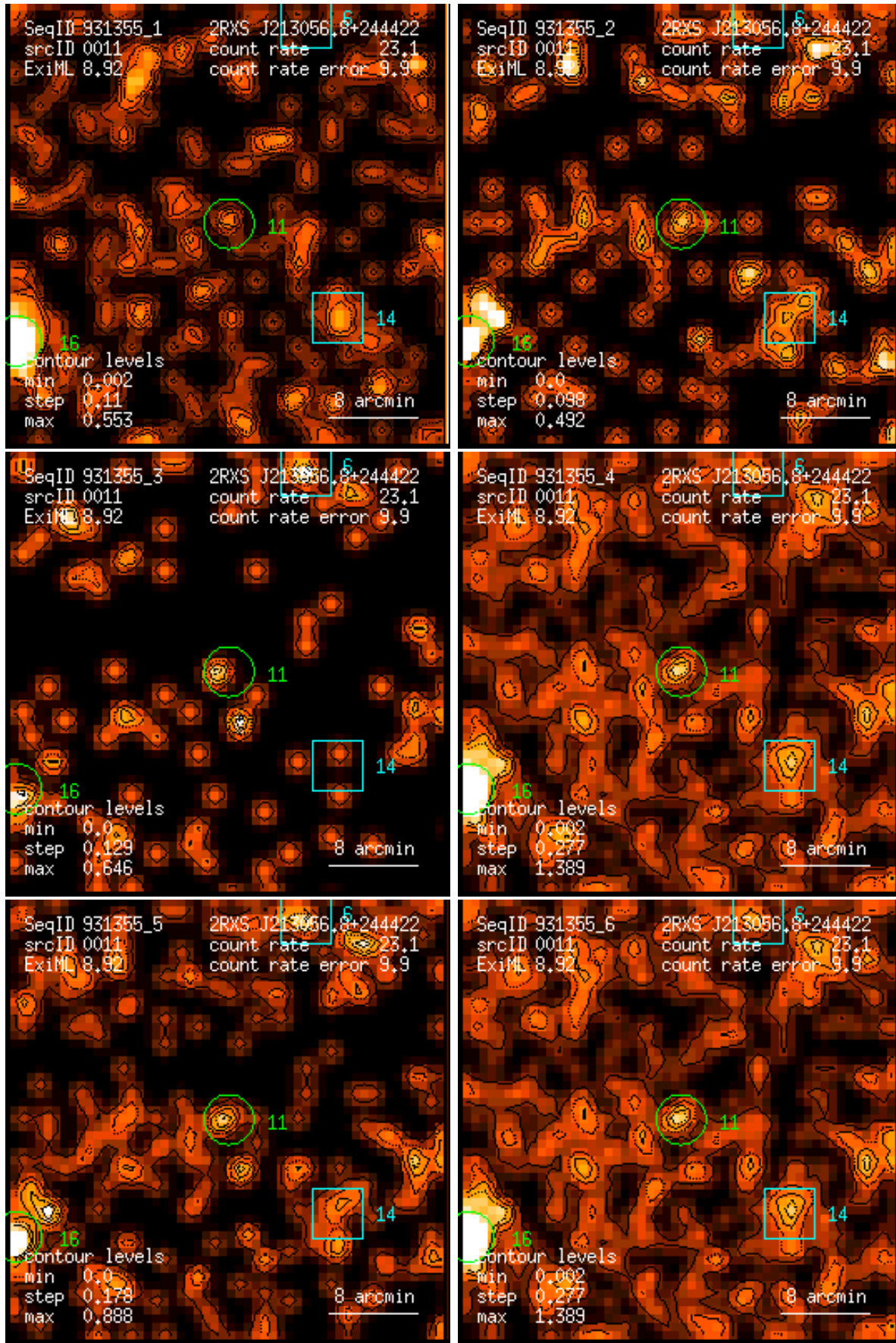
Figure 11: RASS 931355: detection 0011: band rate images, Gaussian filter: (1) PSPC channels 11 – 41, (2) 52 – 90, (3) 91 – 201, (4) 11 – 235, (5) 52 – 201, (6) 11 – 201. Broad band rates in counts/ks. Band rate contour levels in counts/ks/arcmin 2 .
