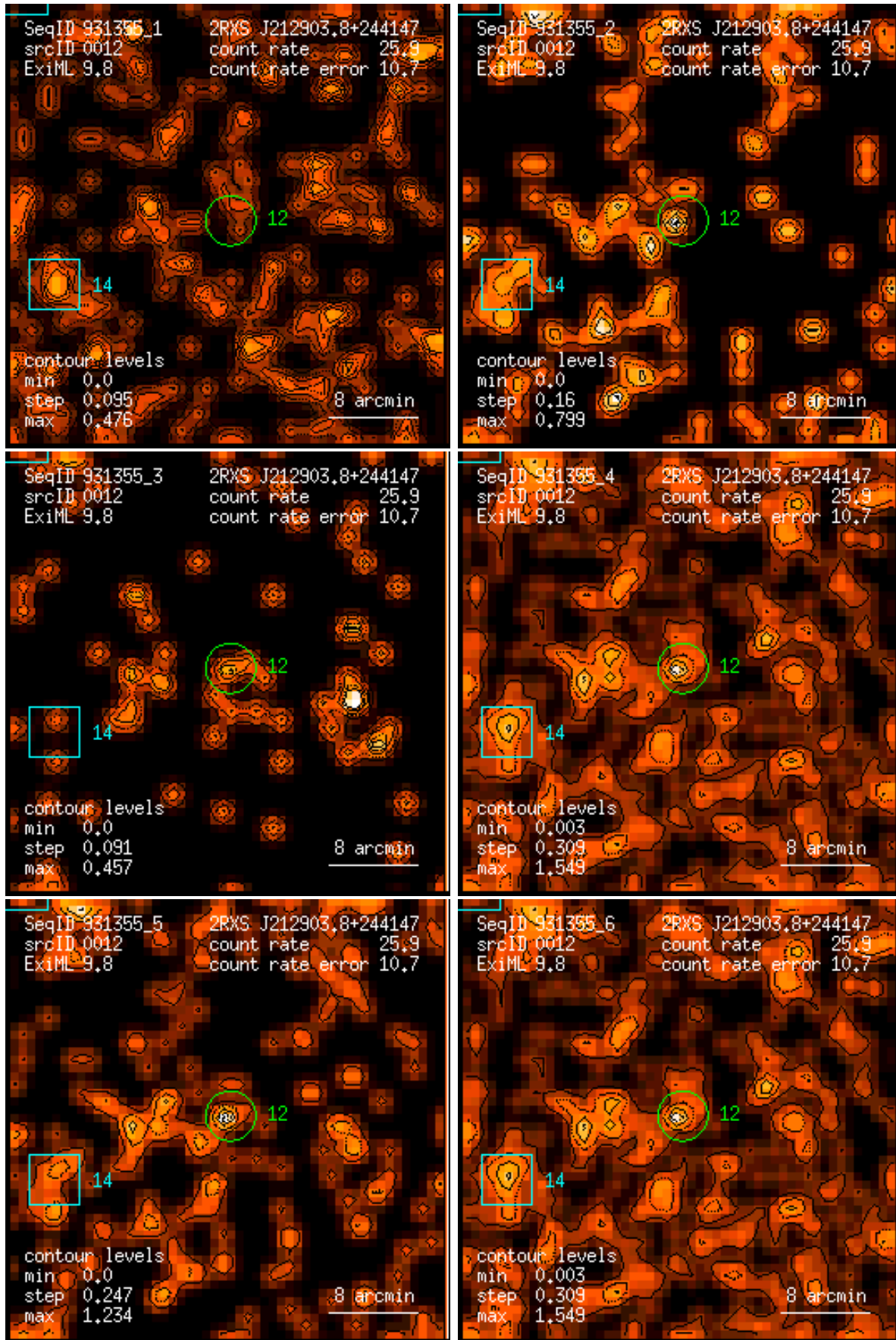
Figure 12: RASS 931355: detection 0012: band rate images, Gaussian filter: (1) PSPC channels 11 – 41, (2) 52 – 90, (3) 91 – 201, (4) 11 – 235, (5) 52 – 201, (6) 11 – 201. Broad band rates in counts/ks. Band rate contour levels in counts/ks/arcmin 2 .
