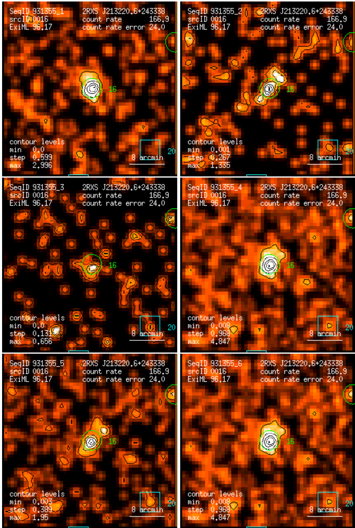
Figure 16: RASS 931355: detection 0016: band rate images, Gaussian filter: (1) PSPC channels 11 – 41, (2) 52 – 90, (3) 91 – 201, (4) 11 – 235, (5) 52 – 201, (6) 11 – 201. Broad band rates in counts/ks. Band rate contour levels in counts/ks/arcmin 2 .
