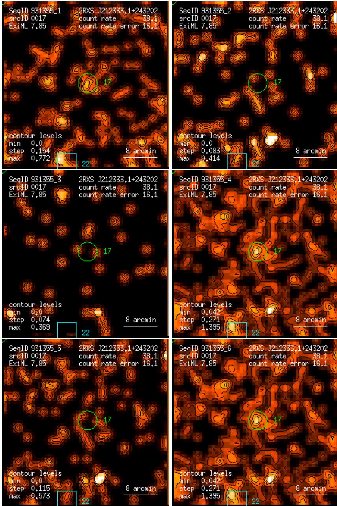
Figure 17: RASS 931355: detection 0017: band rate images, Gaussian filter: (1) PSPC channels 11 – 41, (2) 52 – 90, (3) 91 – 201, (4) 11 – 235, (5) 52 – 201, (6) 11 – 201. Broad band rates in counts/ks. Band rate contour levels in counts/ks/arcmin 2 .
