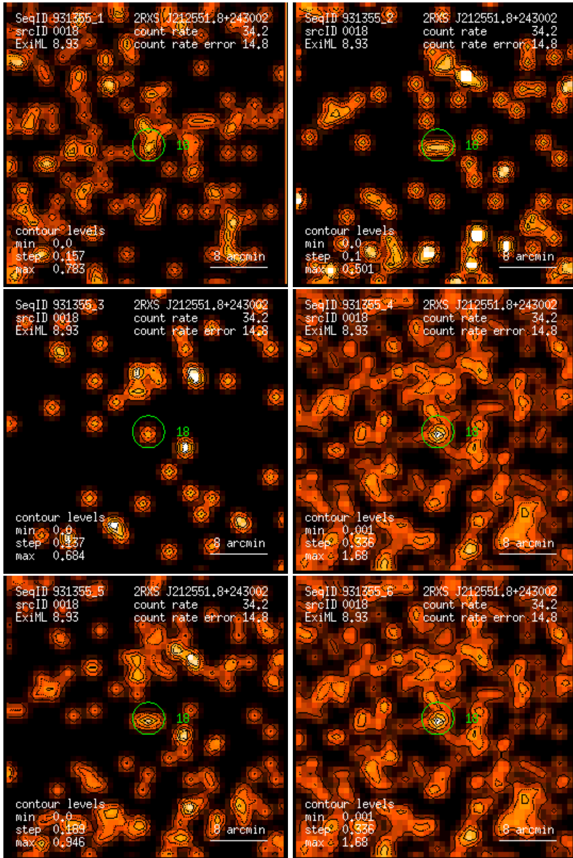
Figure 18: RASS 931355: detection 0018: band rate images, Gaussian filter: (1) PSPC channels 11 – 41, (2) 52 – 90, (3) 91 – 201, (4) 11 – 235, (5) 52 – 201, (6) 11 – 201. Broad band rates in counts/ks. Band rate contour levels in counts/ks/arcmin 2 .
