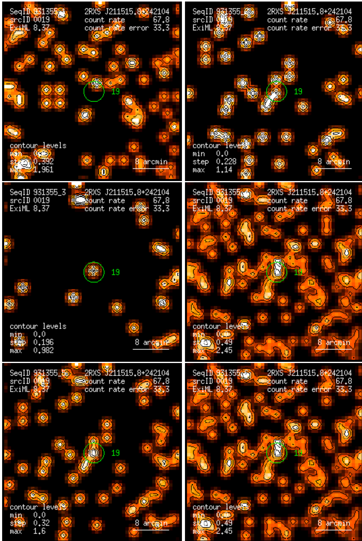
Figure 19: RASS 931355: detection 0019: band rate images, Gaussian filter: (1) PSPC channels 11 – 41, (2) 52 – 90, (3) 91 – 201, (4) 11 – 235, (5) 52 – 201, (6) 11 – 201. Broad band rates in counts/ks. Band rate contour levels in counts/ks/arcmin 2 .
