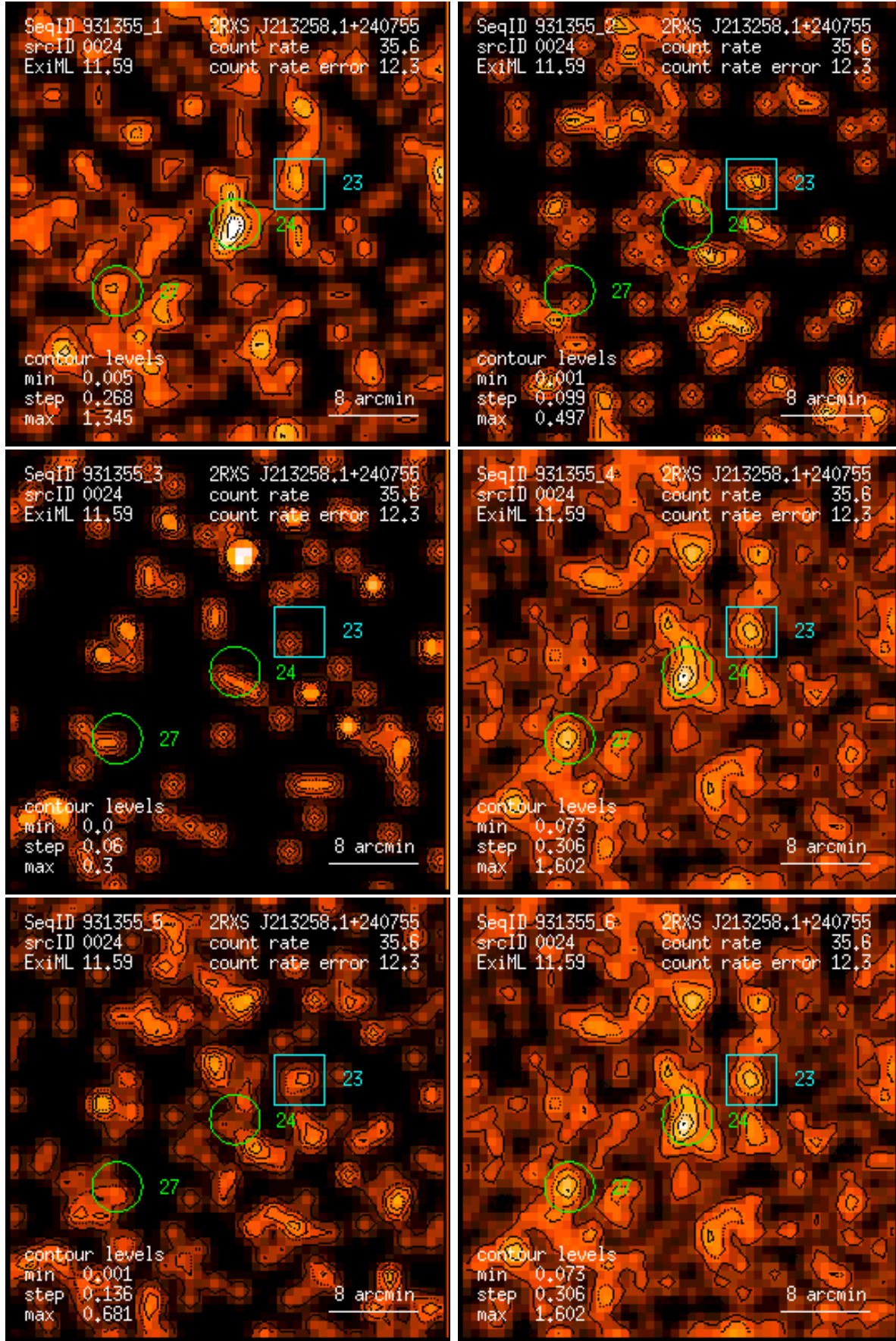
Figure 24: RASS 931355: detection 0024: band rate images, Gaussian filter: (1) PSPC channels 11 – 41, (2) 52 – 90, (3) 91 – 201, (4) 11 – 235, (5) 52 – 201, (6) 11 – 201. Broad band rates in counts/ks. Band rate contour levels in counts/ks/arcmin 2 .
