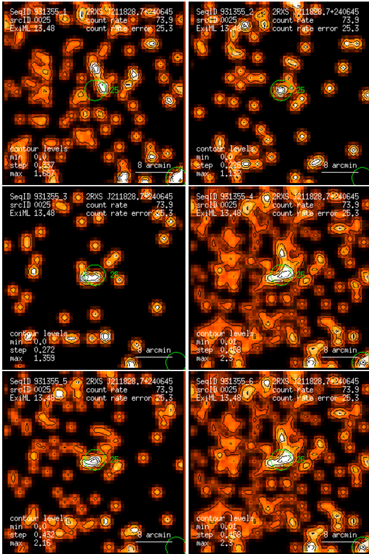
Figure 25: RASS 931355: detection 0025: band rate images, Gaussian filter: (1) PSPC channels 11 – 41, (2) 52 – 90, (3) 91 – 201, (4) 11 – 235, (5) 52 – 201, (6) 11 – 201. Broad band rates in counts/ks. Band rate contour levels in counts/ks/arcmin 2 .
