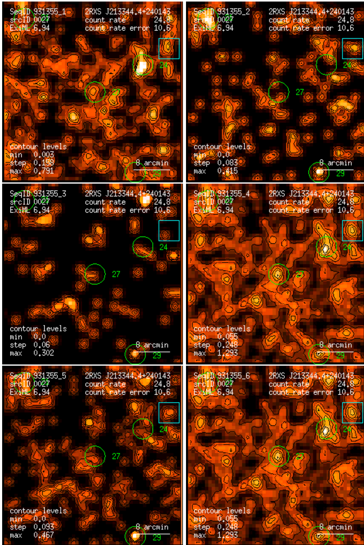
Figure 27: RASS 931355: detection 0027: band rate images, Gaussian filter: (1) PSPC channels 11 – 41, (2) 52 – 90, (3) 91 – 201, (4) 11 – 235, (5) 52 – 201, (6) 11 – 201. Broad band rates in counts/ks. Band rate contour levels in counts/ks/arcmin 2 .
