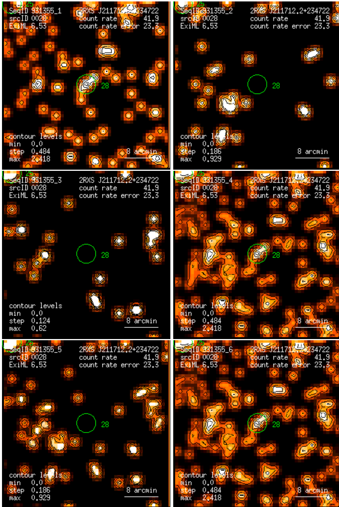
Figure 28: RASS 931355: detection 0028: band rate images, Gaussian filter: (1) PSPC channels 11 – 41, (2) 52 – 90, (3) 91 – 201, (4) 11 – 235, (5) 52 – 201, (6) 11 – 201. Broad band rates in counts/ks. Band rate contour levels in counts/ks/arcmin 2 .
