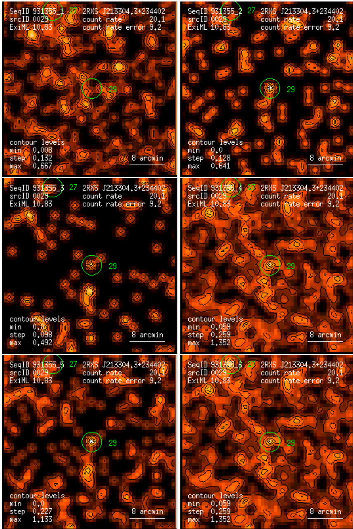
Figure 29: RASS 931355: detection 0029: band rate images, Gaussian filter: (1) PSPC channels 11 – 41, (2) 52 – 90, (3) 91 – 201, (4) 11 – 235, (5) 52 – 201, (6) 11 – 201. Broad band rates in counts/ks. Band rate contour levels in counts/ks/arcmin 2 .
