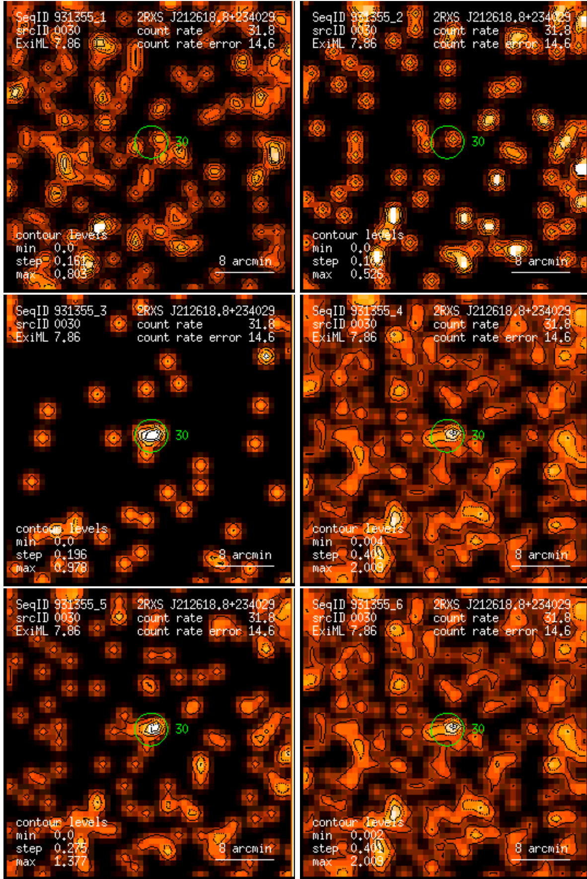
Figure 30: RASS 931355: detection 0030: band rate images, Gaussian filter: (1) PSPC channels 11 – 41, (2) 52 – 90, (3) 91 – 201, (4) 11 – 235, (5) 52 – 201, (6) 11 – 201. Broad band rates in counts/ks. Band rate contour levels in counts/ks/arcmin 2 .
