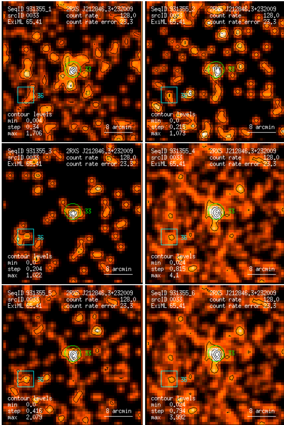
Figure 33: RASS 931355: detection 0033: band rate images, Gaussian filter: (1) PSPC channels 11 – 41, (2) 52 – 90, (3) 91 – 201, (4) 11 – 235, (5) 52 – 201, (6) 11 – 201. Broad band rates in counts/ks. Band rate contour levels in counts/ks/arcmin 2 .
