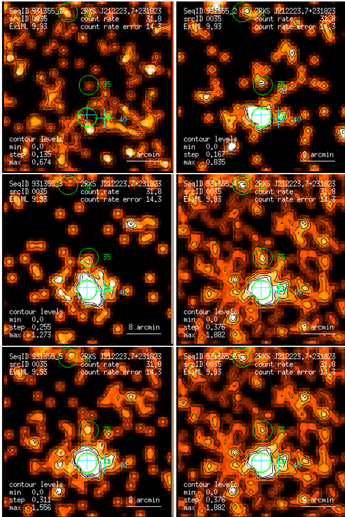
Figure 35: RASS 931355: detection 0035: band rate images, Gaussian filter: (1) PSPC channels 11 – 41, (2) 52 – 90, (3) 91 – 201, (4) 11 – 235, (5) 52 – 201, (6) 11 – 201. Broad band rates in counts/ks. Band rate contour levels in counts/ks/arcmin 2 .
