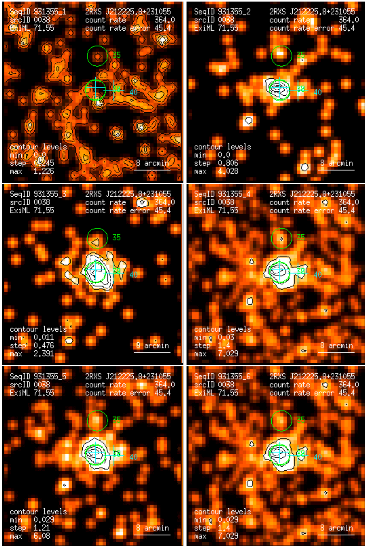
Figure 38: RASS 931355: detection 0038: band rate images, Gaussian filter: (1) PSPC channels 11 – 41, (2) 52 – 90, (3) 91 – 201, (4) 11 – 235, (5) 52 – 201, (6) 11 – 201. Broad band rates in counts/ks. Band rate contour levels in counts/ks/arcmin 2 .
