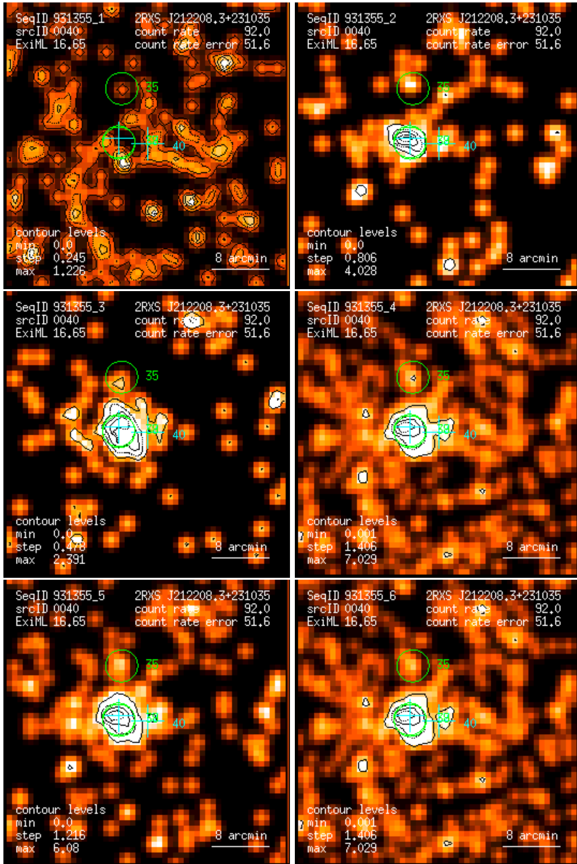
Figure 40: RASS 931355: detection 0040: band rate images, Gaussian filter: (1) PSPC channels 11 – 41, (2) 52 – 90, (3) 91 – 201, (4) 11 – 235, (5) 52 – 201, (6) 11 – 201. Broad band rates in counts/ks. Band rate contour levels in counts/ks/arcmin 2 .
