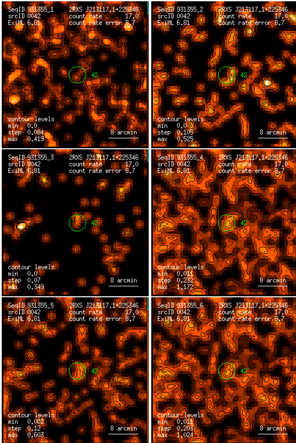
Figure 42: RASS 931355: detection 0042: band rate images, Gaussian filter: (1) PSPC channels 11 – 41, (2) 52 – 90, (3) 91 – 201, (4) 11 – 235, (5) 52 – 201, (6) 11 – 201. Broad band rates in counts/ks. Band rate contour levels in counts/ks/arcmin 2 .
