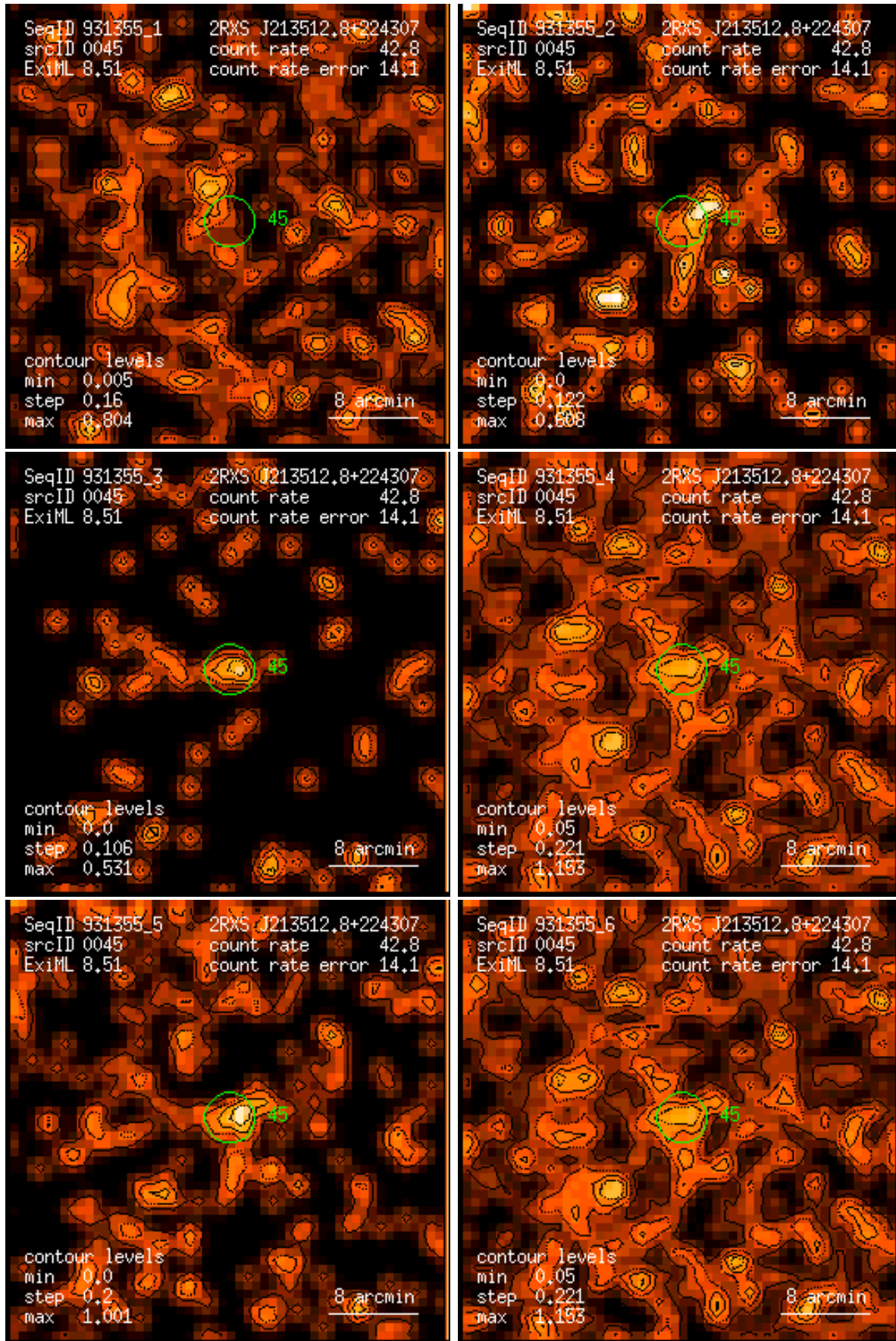
Figure 45: RASS 931355: detection 0045: band rate images, Gaussian filter: (1) PSPC channels 11 – 41, (2) 52 – 90, (3) 91 – 201, (4) 11 – 235, (5) 52 – 201, (6) 11 – 201. Broad band rates in counts/ks. Band rate contour levels in counts/ks/arcmin 2 .
