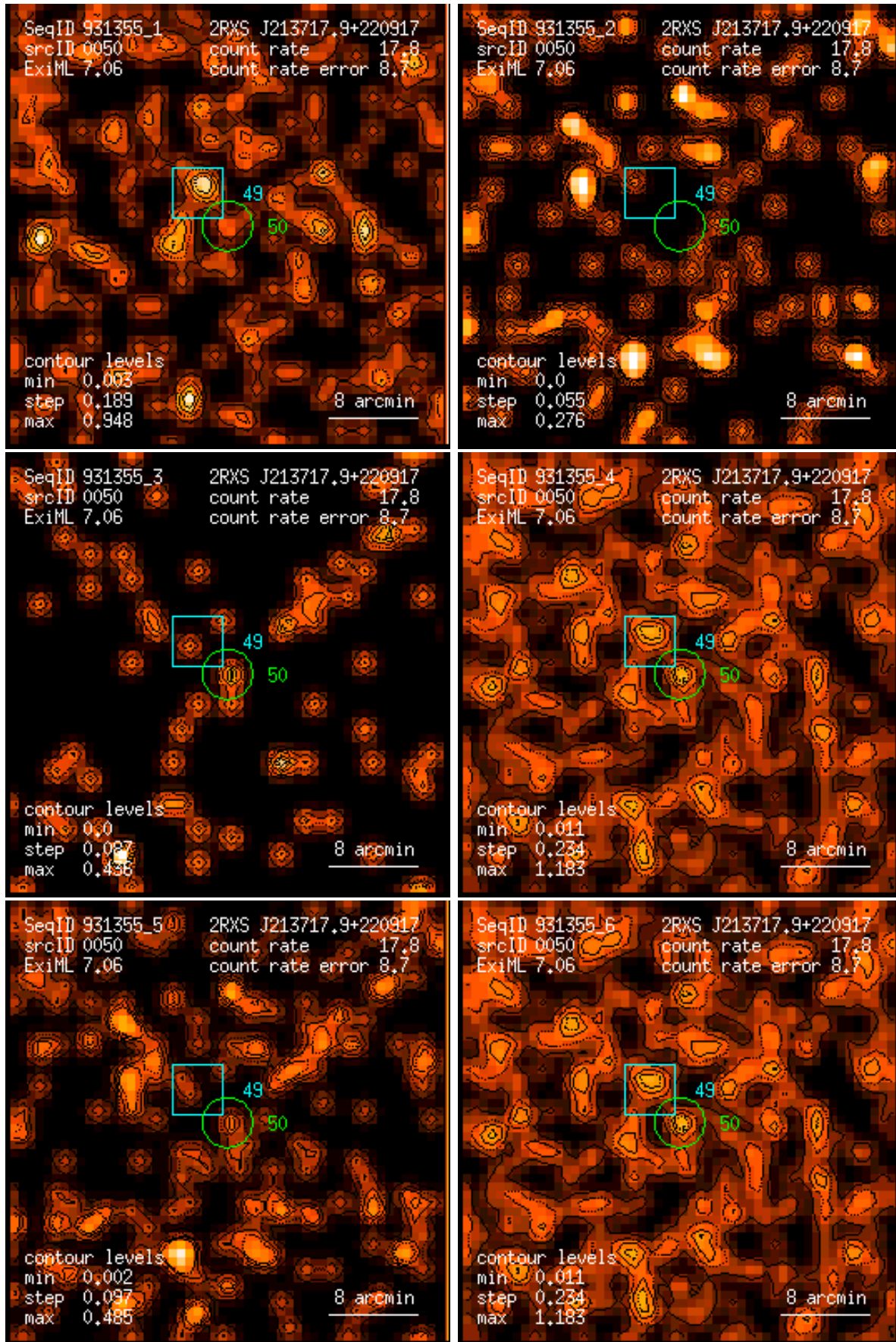
Figure 50: RASS 931355: detection 0050: band rate images, Gaussian filter: (1) PSPC channels 11 – 41, (2) 52 – 90, (3) 91 – 201, (4) 11 – 235, (5) 52 – 201, (6) 11 – 201. Broad band rates in counts/ks. Band rate contour levels in counts/ks/arcmin 2 .
