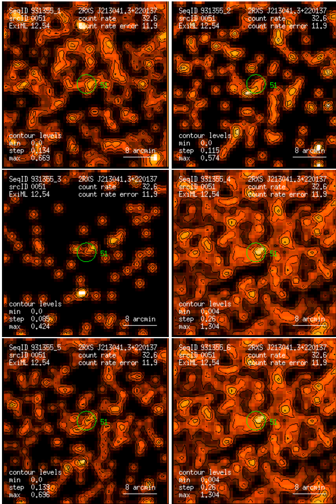
Figure 51: RASS 931355: detection 0051: band rate images, Gaussian filter: (1) PSPC channels 11 – 41, (2) 52 – 90, (3) 91 – 201, (4) 11 – 235, (5) 52 – 201, (6) 11 – 201. Broad band rates in counts/ks. Band rate contour levels in counts/ks/arcmin 2 .
