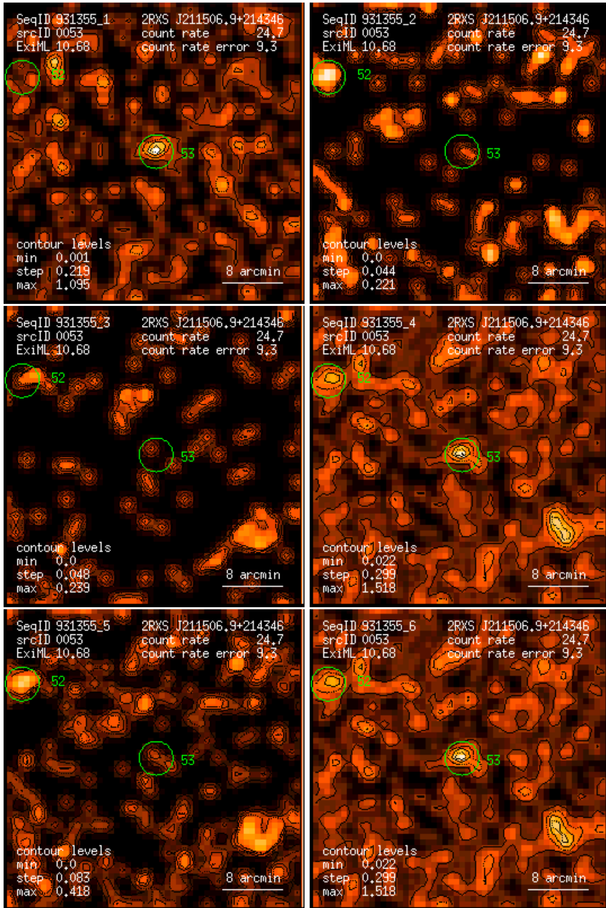
Figure 53: RASS 931355: detection 0053: band rate images, Gaussian filter: (1) PSPC channels 11 – 41, (2) 52 – 90, (3) 91 – 201, (4) 11 – 235, (5) 52 – 201, (6) 11 – 201. Broad band rates in counts/ks. Band rate contour levels in counts/ks/arcmin 2 .
