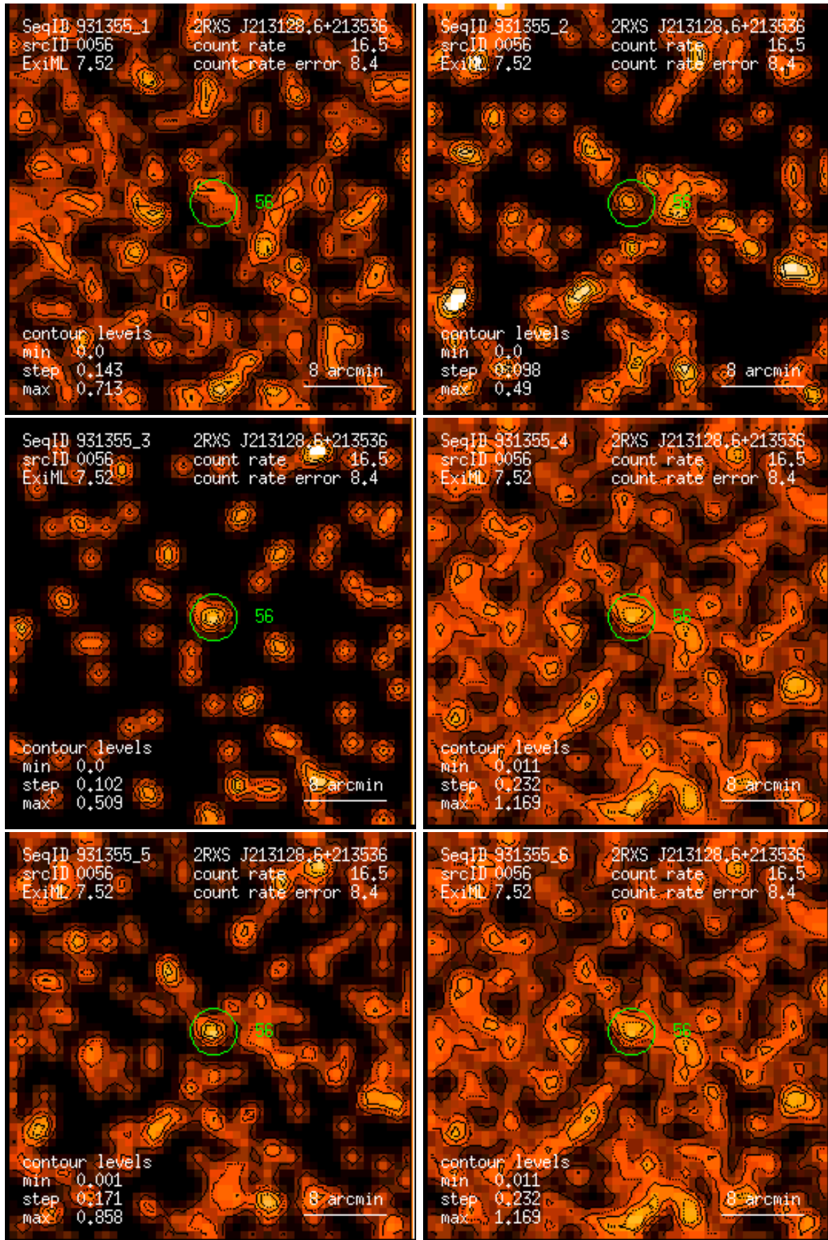
Figure 56: RASS 931355: detection 0056: band rate images, Gaussian filter: (1) PSPC channels 11 – 41, (2) 52 – 90, (3) 91 – 201, (4) 11 – 235, (5) 52 – 201, (6) 11 – 201. Broad band rates in counts/ks. Band rate contour levels in counts/ks/arcmin 2 .
