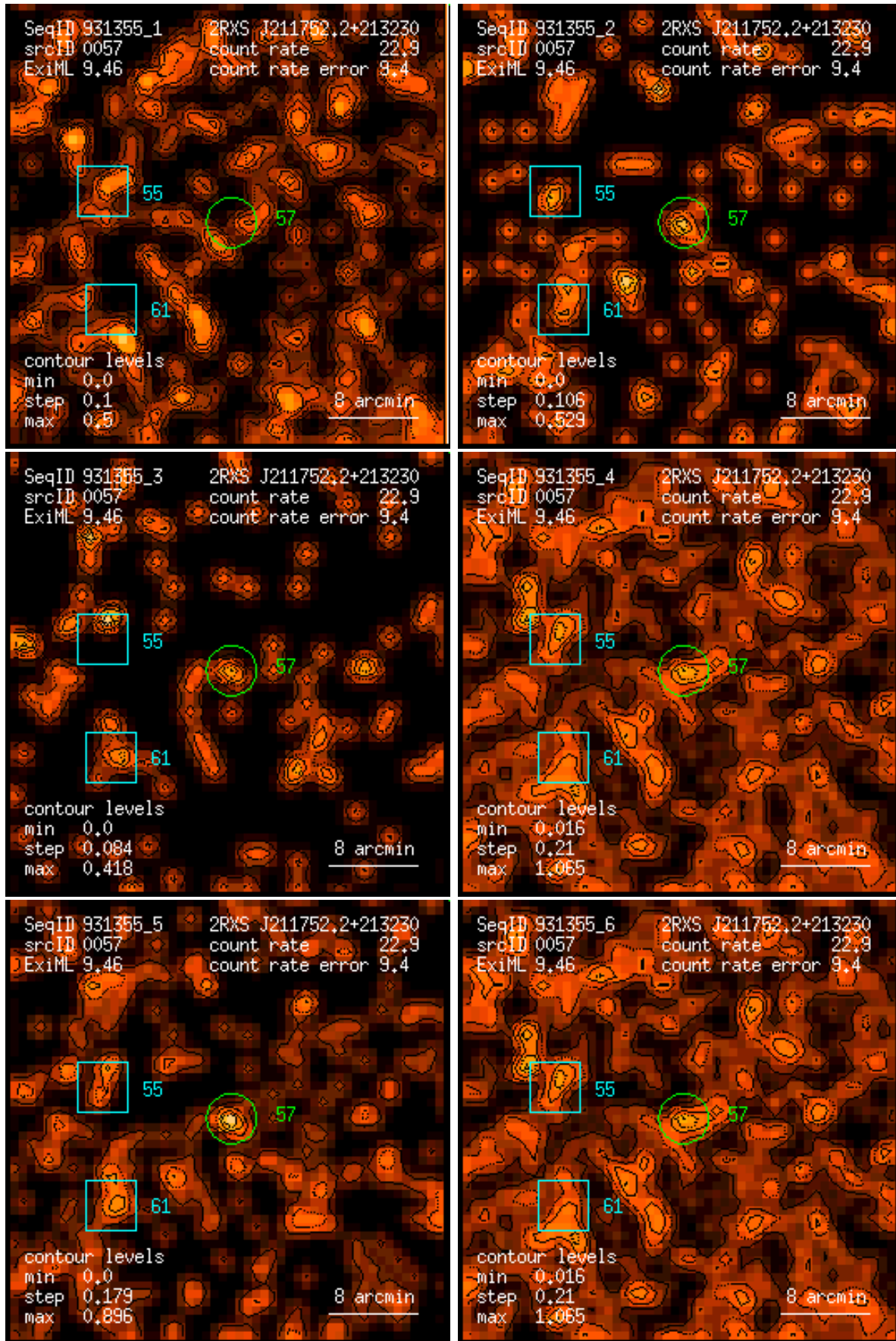
Figure 57: RASS 931355: detection 0057: band rate images, Gaussian filter: (1) PSPC channels 11 – 41, (2) 52 – 90, (3) 91 – 201, (4) 11 – 235, (5) 52 – 201, (6) 11 – 201. Broad band rates in counts/ks. Band rate contour levels in counts/ks/arcmin 2 .
