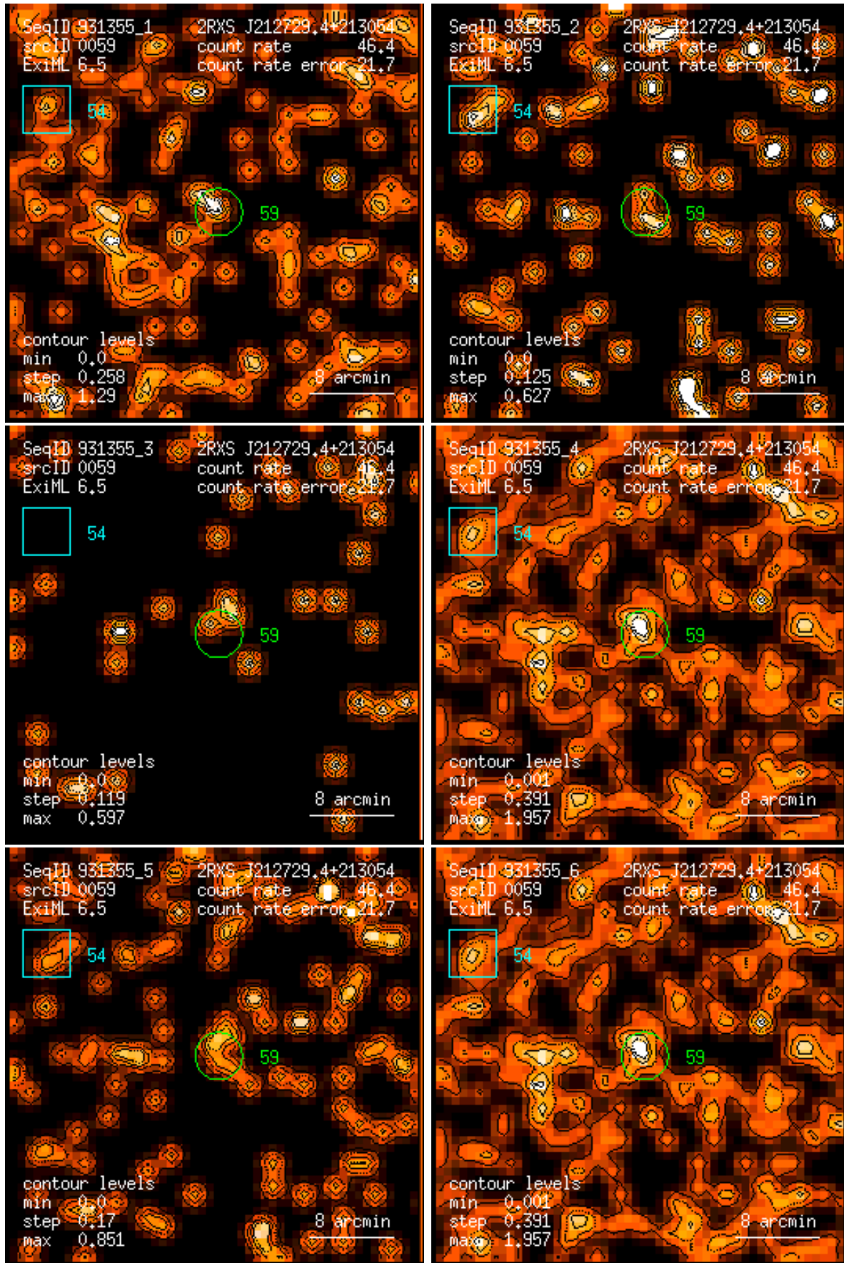
Figure 59: RASS 931355: detection 0059: band rate images, Gaussian filter: (1) PSPC channels 11 – 41, (2) 52 – 90, (3) 91 – 201, (4) 11 – 235, (5) 52 – 201, (6) 11 – 201. Broad band rates in counts/ks. Band rate contour levels in counts/ks/arcmin 2 .
