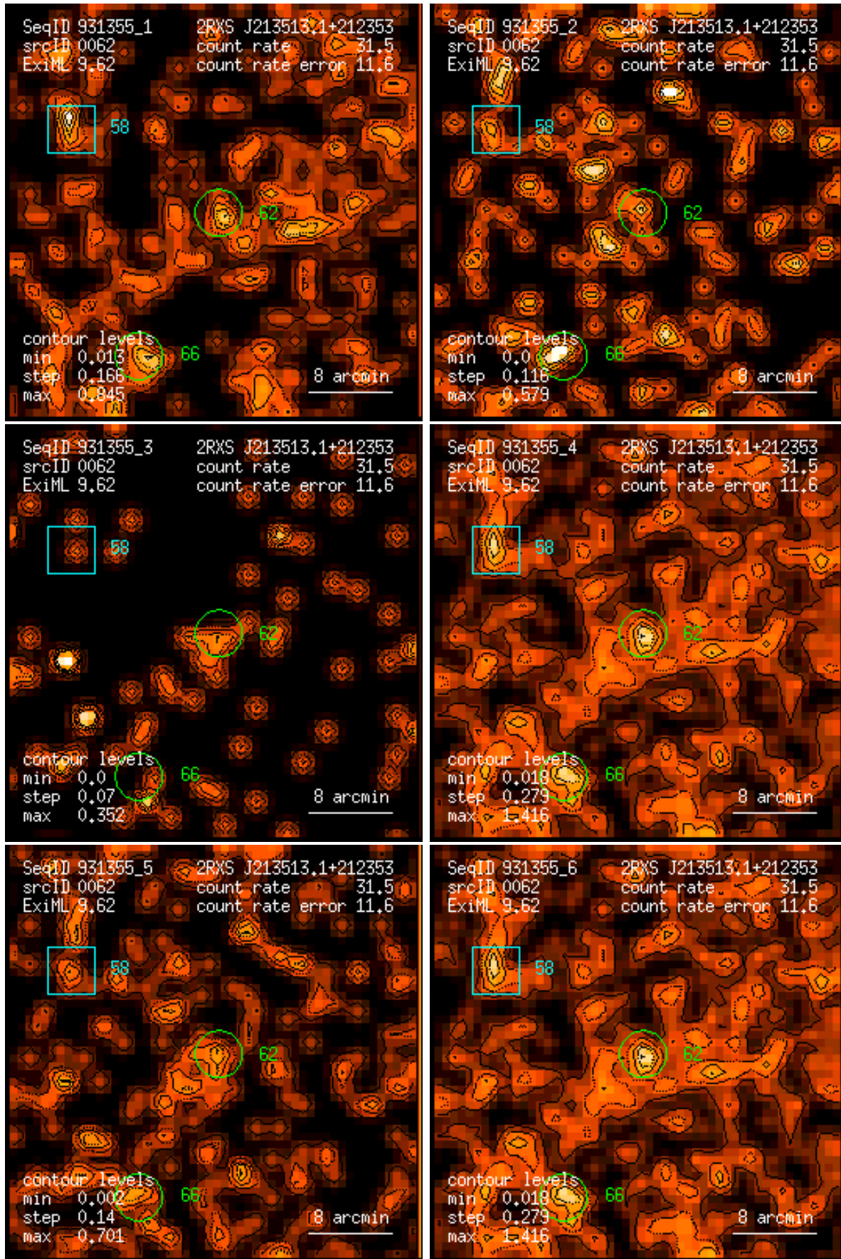
Figure 62: RASS 931355: detection 0062: band rate images, Gaussian filter: (1) PSPC channels 11 – 41, (2) 52 – 90, (3) 91 – 201, (4) 11 – 235, (5) 52 – 201, (6) 11 – 201. Broad band rates in counts/ks. Band rate contour levels in counts/ks/arcmin 2 .
