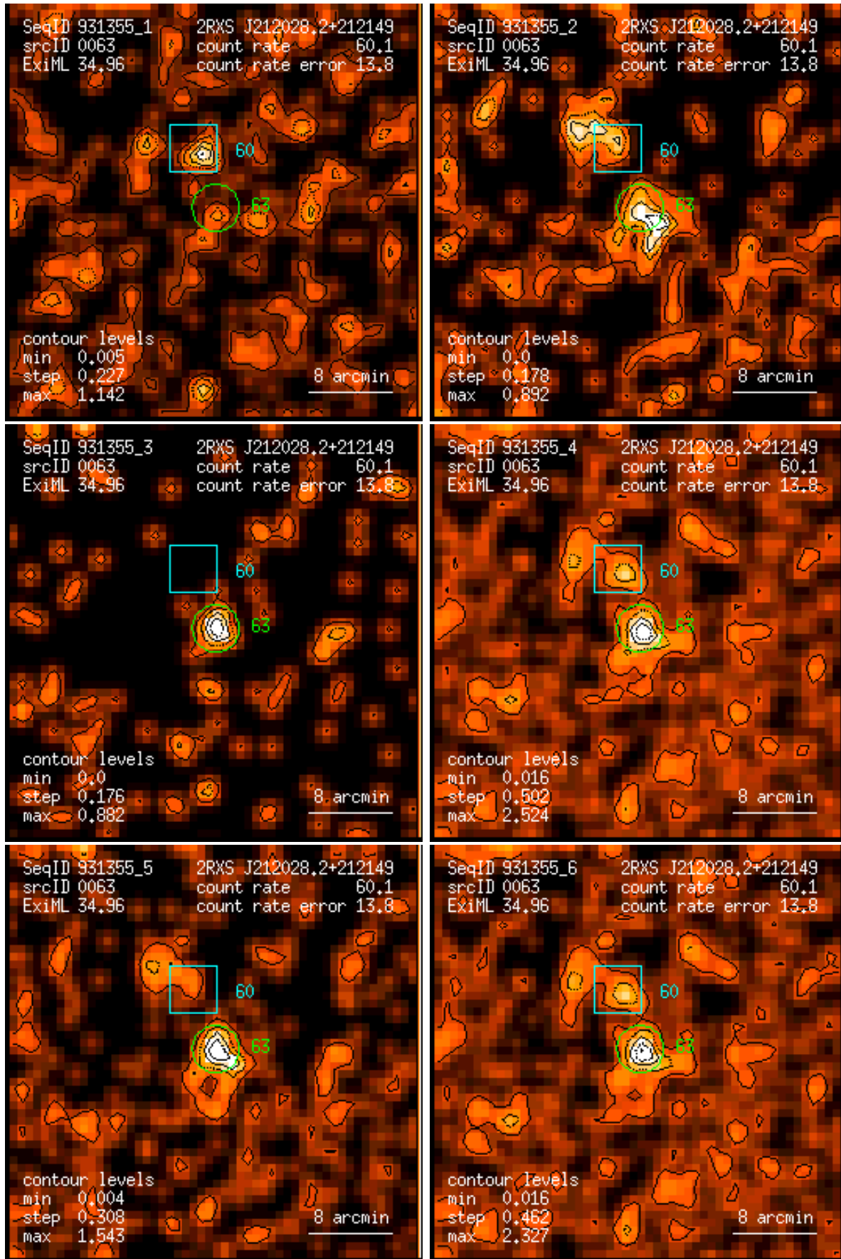
Figure 63: RASS 931355: detection 0063: band rate images, Gaussian filter: (1) PSPC channels 11 – 41, (2) 52 – 90, (3) 91 – 201, (4) 11 – 235, (5) 52 – 201, (6) 11 – 201. Broad band rates in counts/ks. Band rate contour levels in counts/ks/arcmin 2 .
