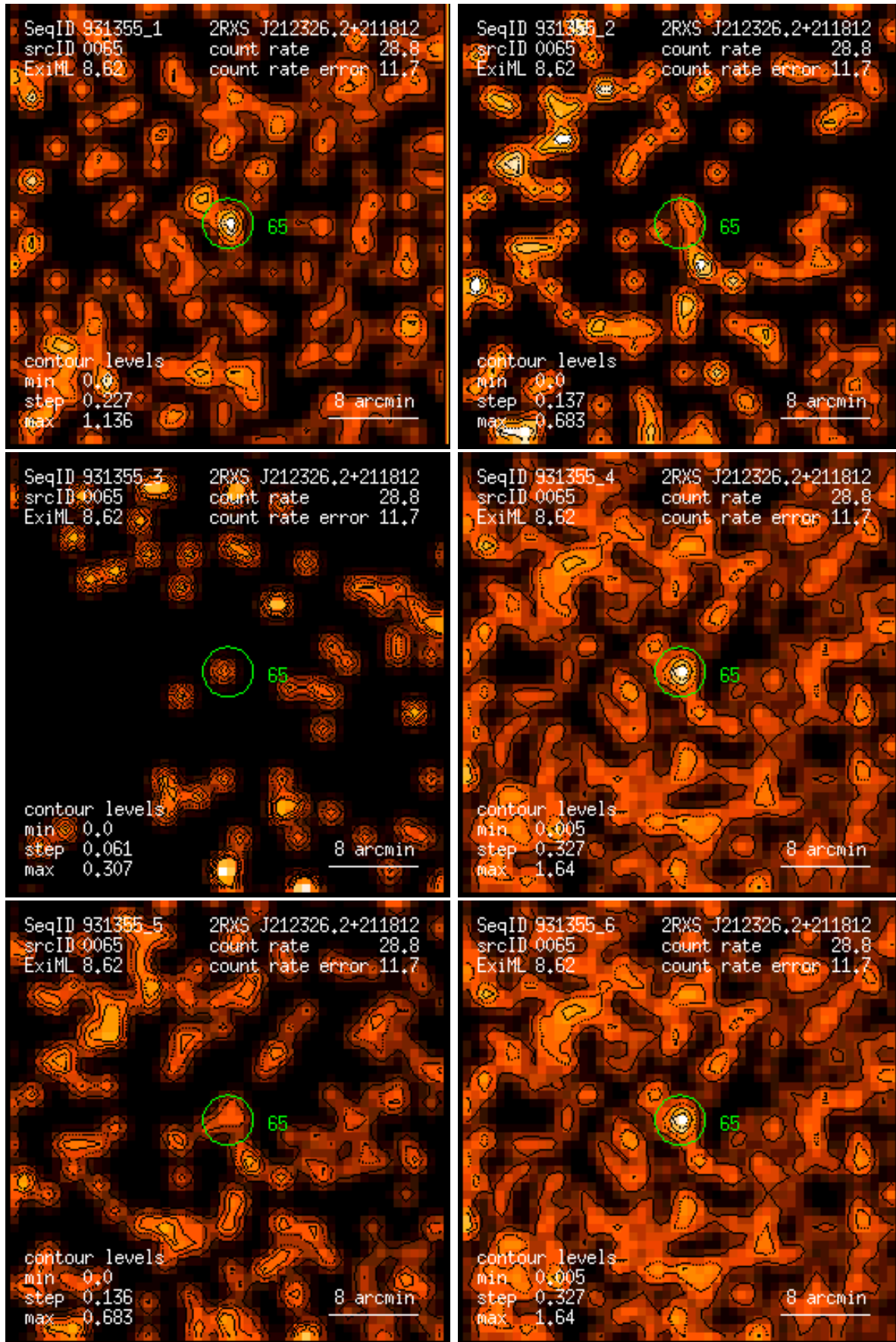
Figure 65: RASS 931355: detection 0065: band rate images, Gaussian filter: (1) PSPC channels 11 – 41, (2) 52 – 90, (3) 91 – 201, (4) 11 – 235, (5) 52 – 201, (6) 11 – 201. Broad band rates in counts/ks. Band rate contour levels in counts/ks/arcmin 2 .
