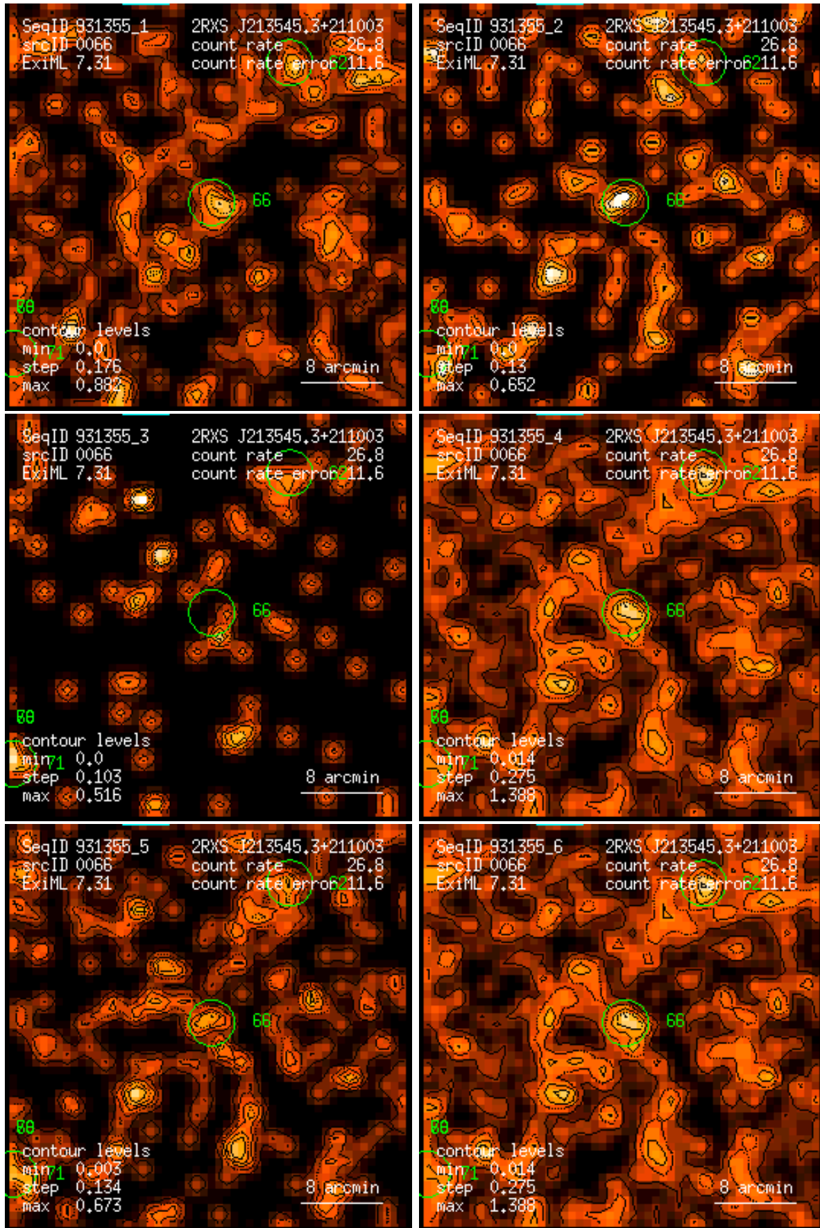
Figure 66: RASS 931355: detection 0066: band rate images, Gaussian filter: (1) PSPC channels 11 – 41, (2) 52 – 90, (3) 91 – 201, (4) 11 – 235, (5) 52 – 201, (6) 11 – 201. Broad band rates in counts/ks. Band rate contour levels in counts/ks/arcmin 2 .
