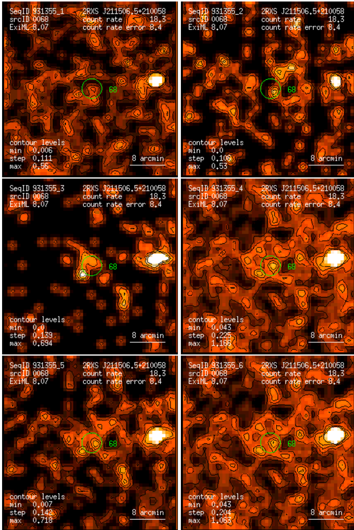
Figure 68: RASS 931355: detection 0068: band rate images, Gaussian filter: (1) PSPC channels 11 – 41, (2) 52 – 90, (3) 91 – 201, (4) 11 – 235, (5) 52 – 201, (6) 11 – 201. Broad band rates in counts/ks. Band rate contour levels in counts/ks/arcmin 2 .
