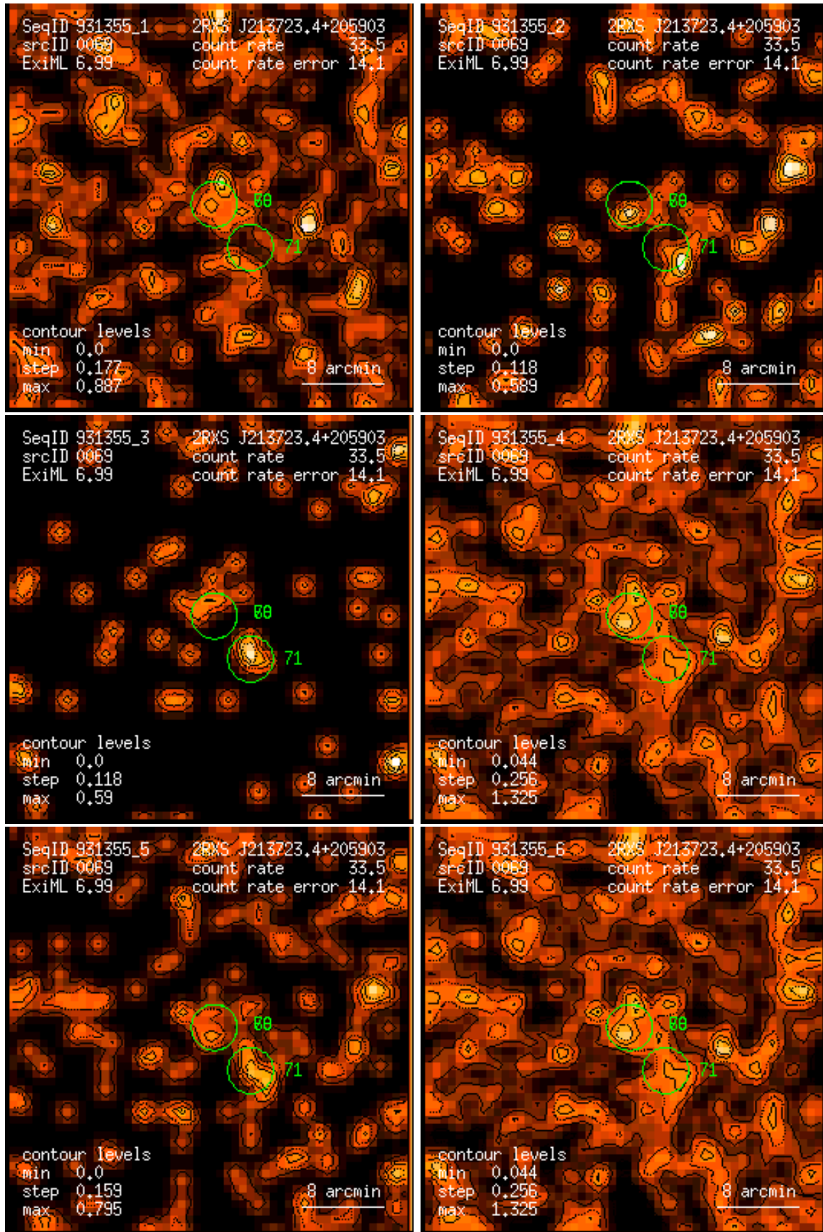
Figure 69: RASS 931355: detection 0069: band rate images, Gaussian filter: (1) PSPC channels 11 – 41, (2) 52 – 90, (3) 91 – 201, (4) 11 – 235, (5) 52 – 201, (6) 11 – 201. Broad band rates in counts/ks. Band rate contour levels in counts/ks/arcmin 2 .
