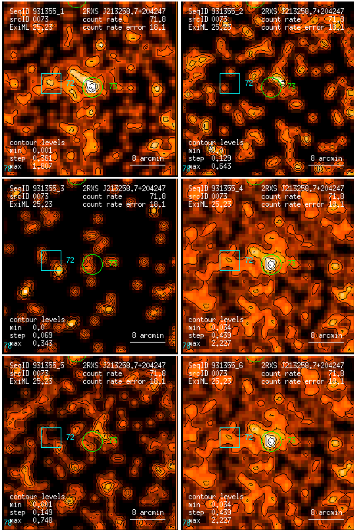
Figure 73: RASS 931355: detection 0073: band rate images, Gaussian filter: (1) PSPC channels 11 – 41, (2) 52 – 90, (3) 91 – 201, (4) 11 – 235, (5) 52 – 201, (6) 11 – 201. Broad band rates in counts/ks. Band rate contour levels in counts/ks/arcmin 2 .
