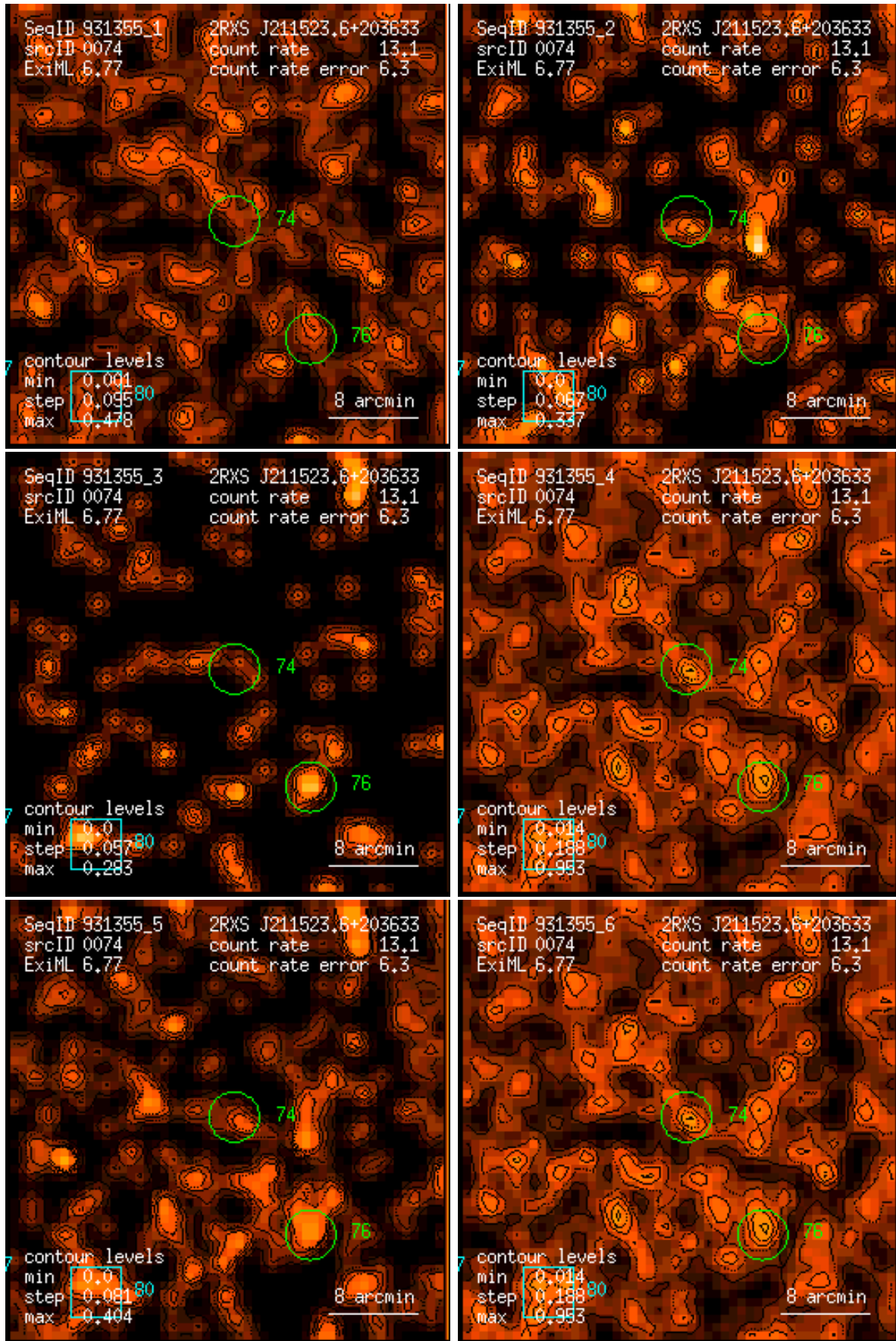
Figure 74: RASS 931355: detection 0074: band rate images, Gaussian filter: (1) PSPC channels 11 – 41, (2) 52 – 90, (3) 91 – 201, (4) 11 – 235, (5) 52 – 201, (6) 11 – 201. Broad band rates in counts/ks. Band rate contour levels in counts/ks/arcmin 2 .
