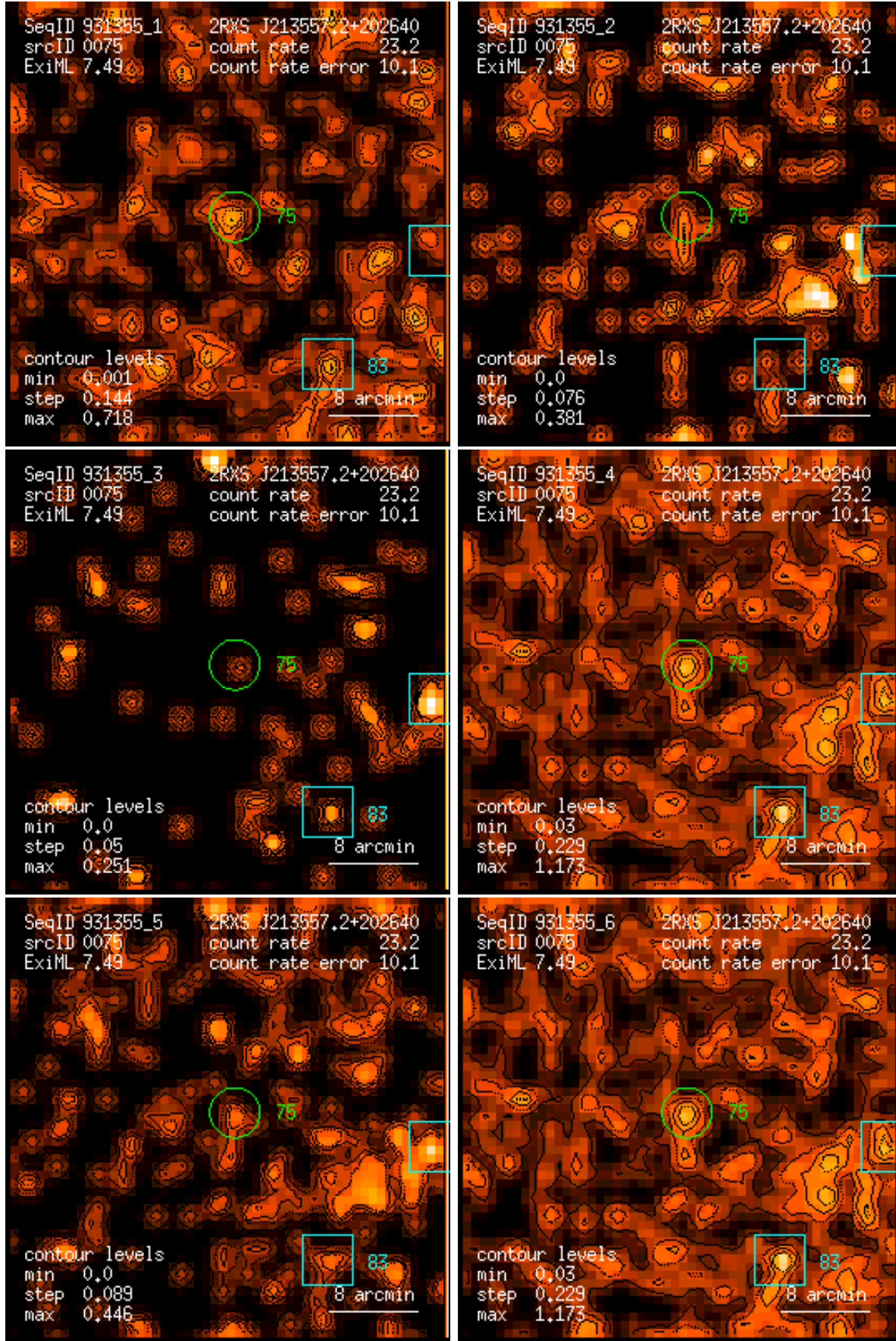
Figure 75: RASS 931355: detection 0075: band rate images, Gaussian filter: (1) PSPC channels 11 – 41, (2) 52 – 90, (3) 91 – 201, (4) 11 – 235, (5) 52 – 201, (6) 11 – 201. Broad band rates in counts/ks. Band rate contour levels in counts/ks/arcmin 2 .
