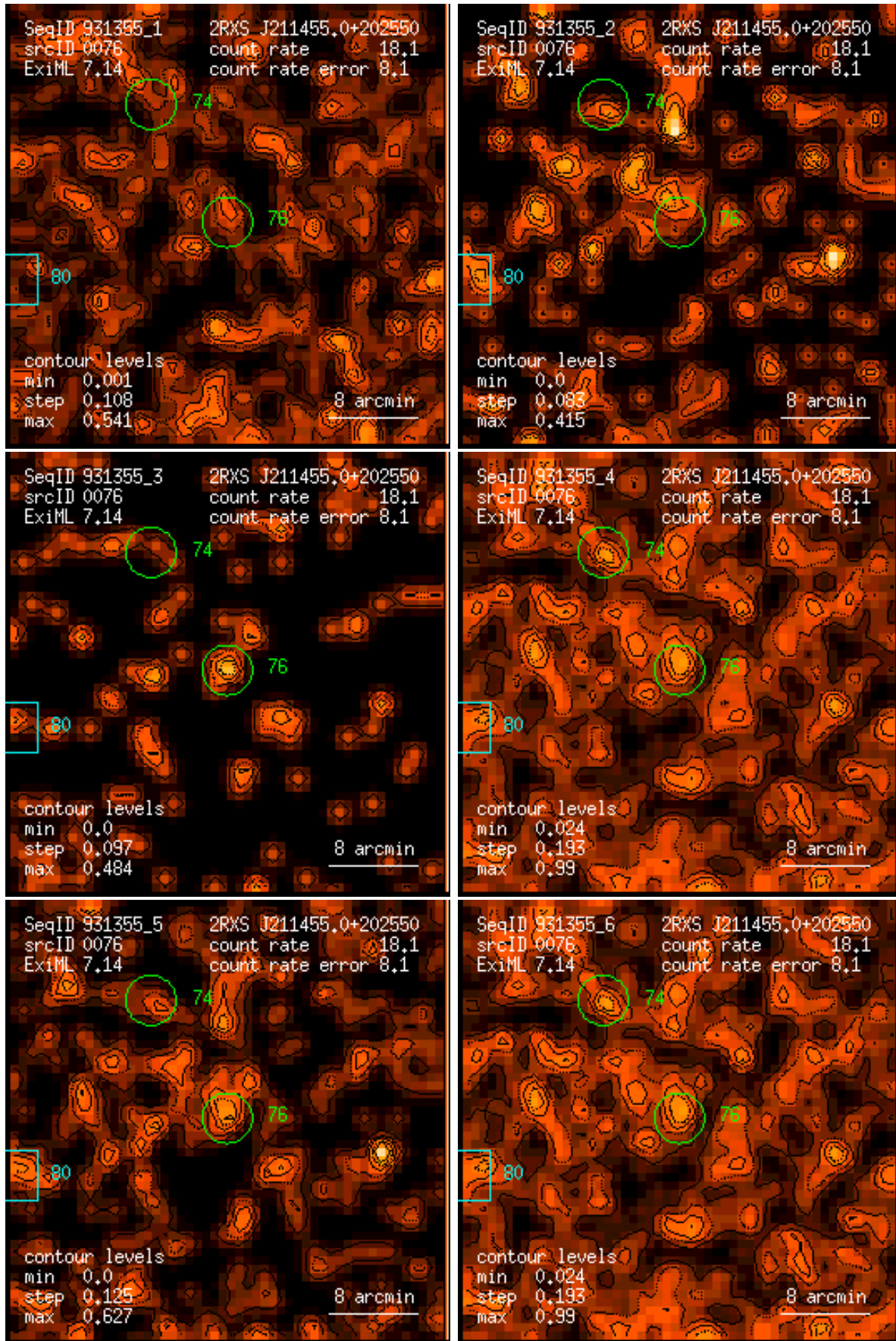
Figure 76: RASS 931355: detection 0076: band rate images, Gaussian filter: (1) PSPC channels 11 – 41, (2) 52 – 90, (3) 91 – 201, (4) 11 – 235, (5) 52 – 201, (6) 11 – 201. Broad band rates in counts/ks. Band rate contour levels in counts/ks/arcmin 2 .
