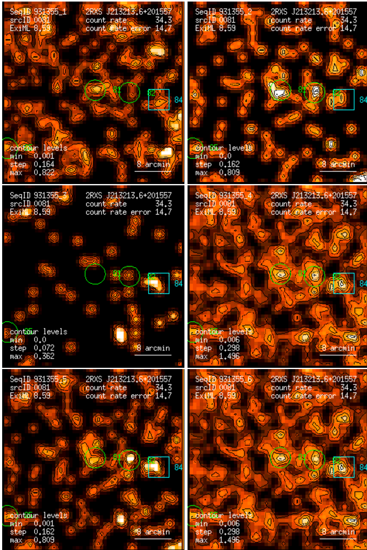
Figure 81: RASS 931355: detection 0081: band rate images, Gaussian filter: (1) PSPC channels 11 – 41, (2) 52 – 90, (3) 91 – 201, (4) 11 – 235, (5) 52 – 201, (6) 11 – 201. Broad band rates in counts/ks. Band rate contour levels in counts/ks/arcmin 2 .
