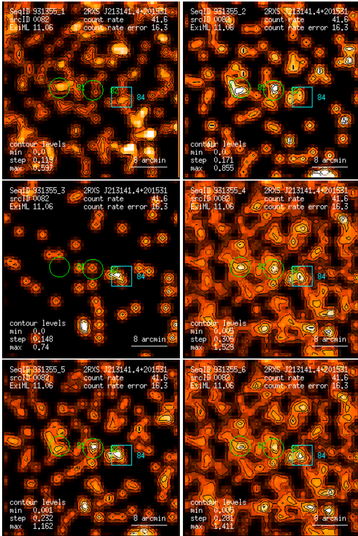
Figure 82: RASS 931355: detection 0082: band rate images, Gaussian filter: (1) PSPC channels 11 – 41, (2) 52 – 90, (3) 91 – 201, (4) 11 – 235, (5) 52 – 201, (6) 11 – 201. Broad band rates in counts/ks. Band rate contour levels in counts/ks/arcmin 2 .
