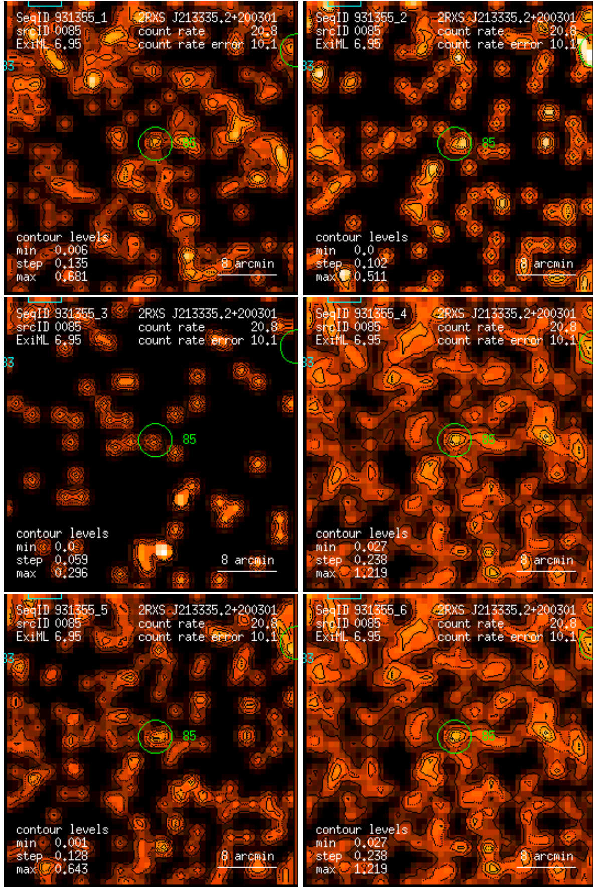
Figure 85: RASS 931355: detection 0085: band rate images, Gaussian filter: (1) PSPC channels 11 – 41, (2) 52 – 90, (3) 91 – 201, (4) 11 – 235, (5) 52 – 201, (6) 11 – 201. Broad band rates in counts/ks. Band rate contour levels in counts/ks/arcmin 2 .
