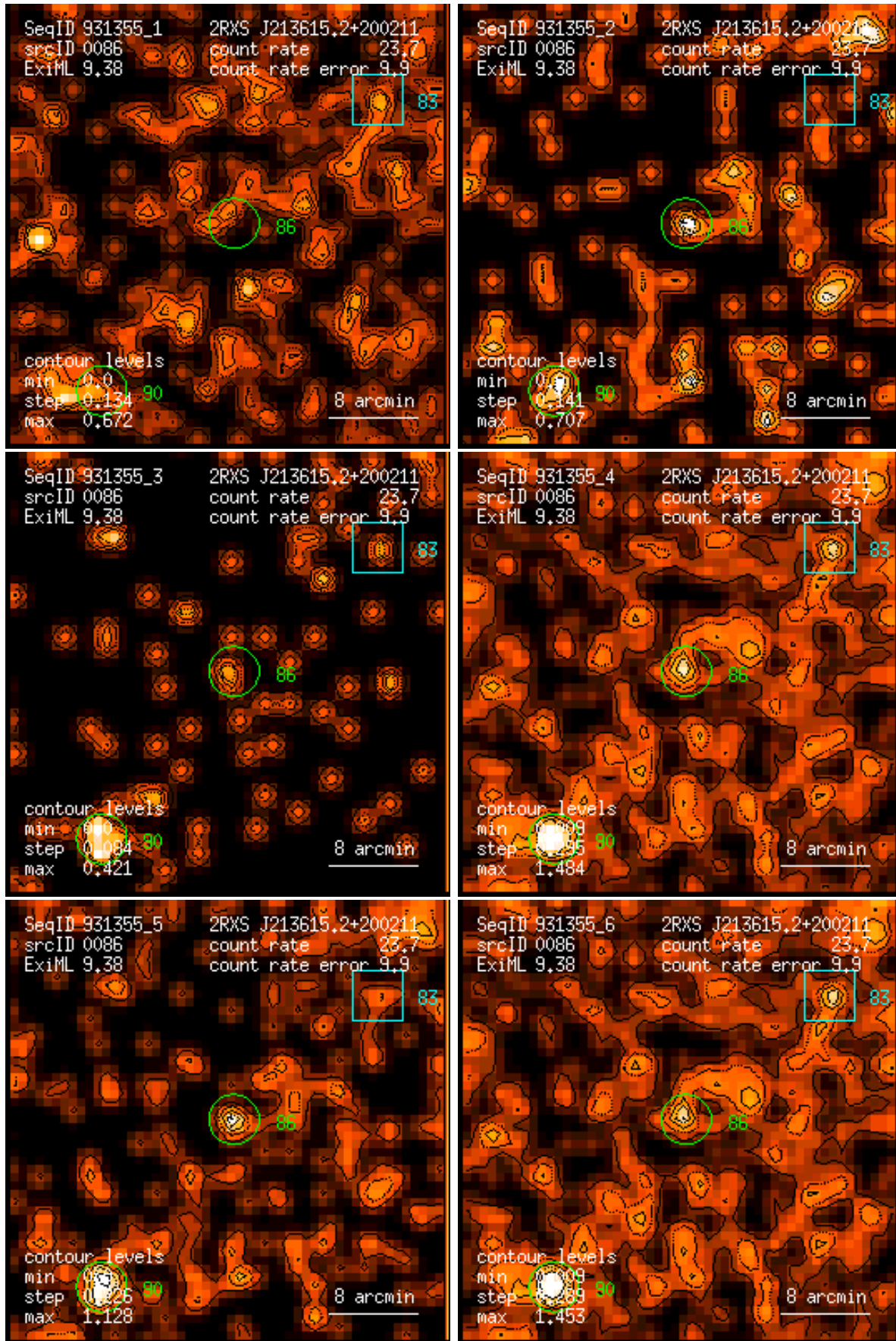
Figure 86: RASS 931355: detection 0086: band rate images, Gaussian filter: (1) PSPC channels 11 – 41, (2) 52 – 90, (3) 91 – 201, (4) 11 – 235, (5) 52 – 201, (6) 11 – 201. Broad band rates in counts/ks. Band rate contour levels in counts/ks/arcmin 2 .
