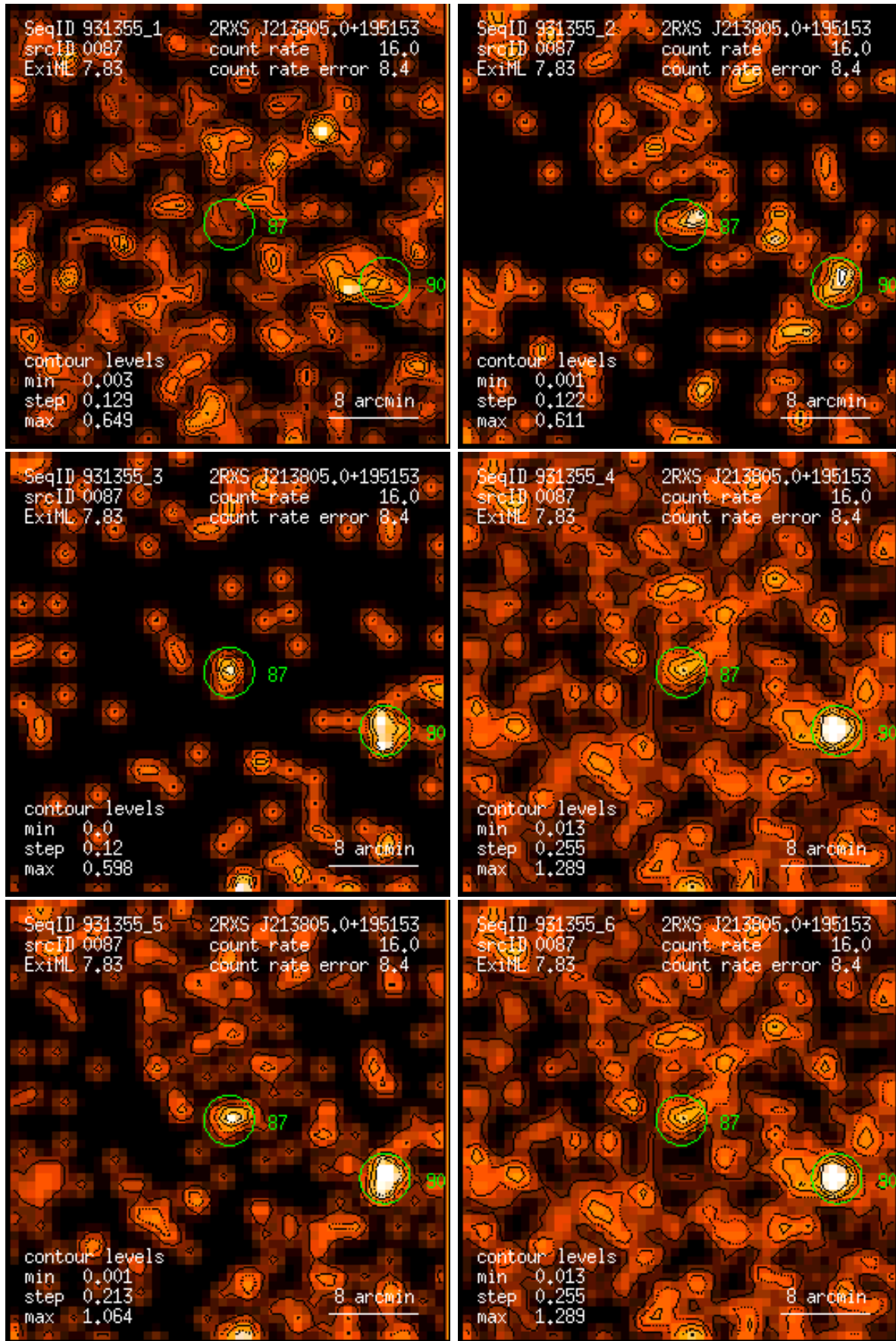
Figure 87: RASS 931355: detection 0087: band rate images, Gaussian filter: (1) PSPC channels 11 – 41, (2) 52 – 90, (3) 91 – 201, (4) 11 – 235, (5) 52 – 201, (6) 11 – 201. Broad band rates in counts/ks. Band rate contour levels in counts/ks/arcmin 2 .
