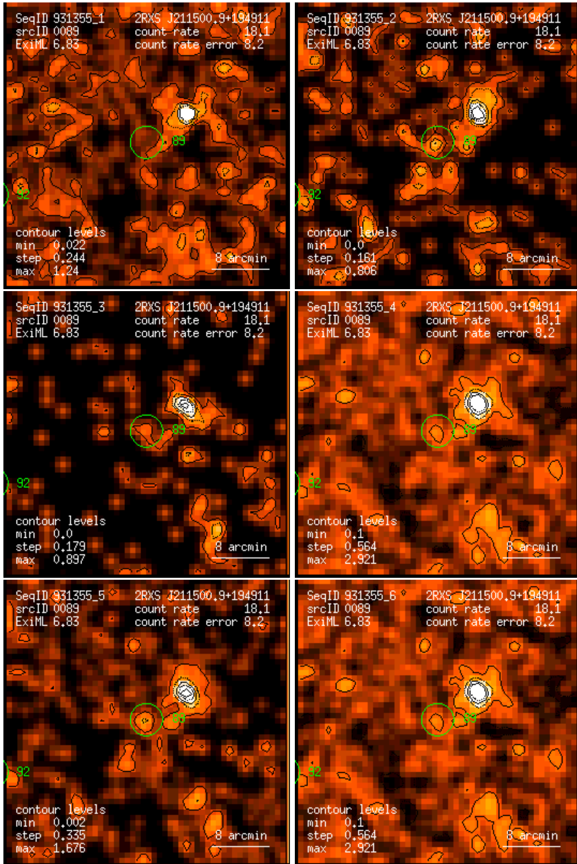
Figure 89: RASS 931355: detection 0089: band rate images, Gaussian filter: (1) PSPC channels 11 – 41, (2) 52 – 90, (3) 91 – 201, (4) 11 – 235, (5) 52 – 201, (6) 11 – 201. Broad band rates in counts/ks. Band rate contour levels in counts/ks/arcmin 2 .
