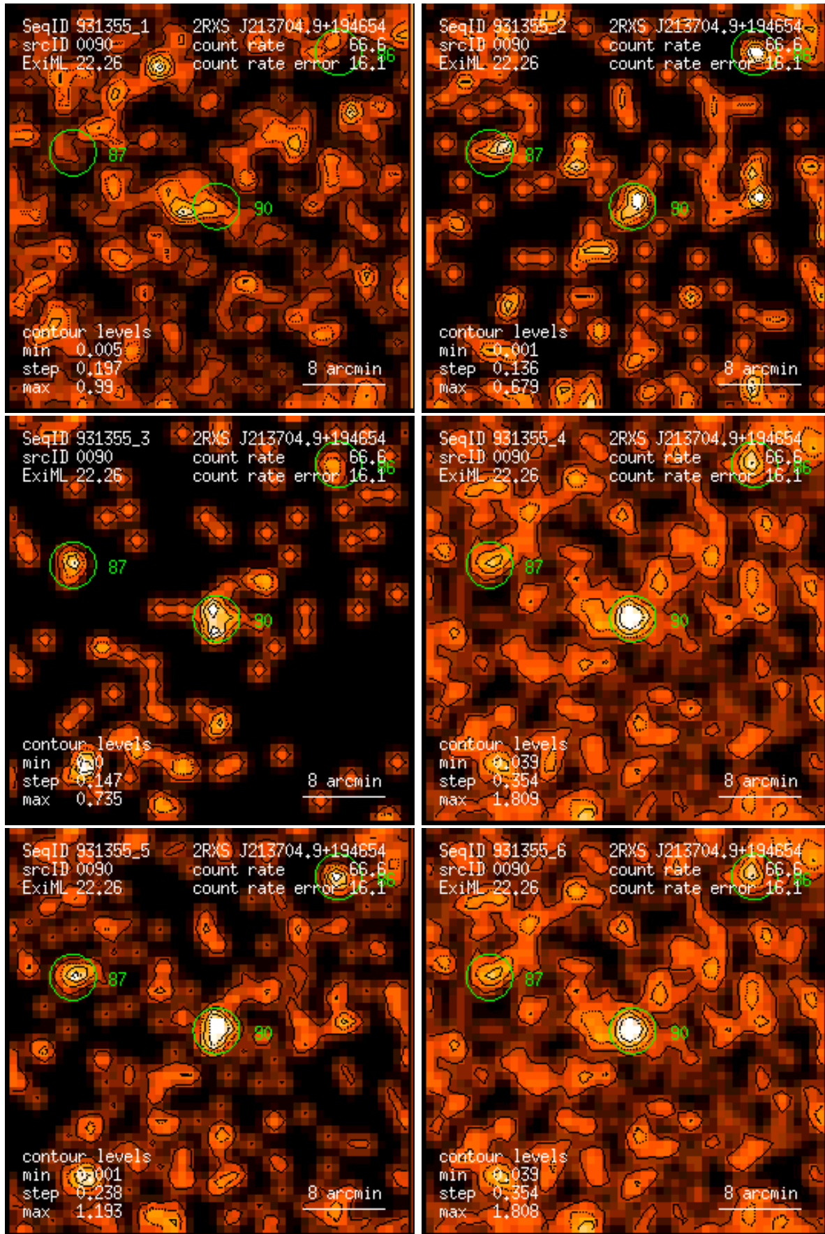
Figure 90: RASS 931355: detection 0090: band rate images, Gaussian filter: (1) PSPC channels 11 – 41, (2) 52 – 90, (3) 91 – 201, (4) 11 – 235, (5) 52 – 201, (6) 11 – 201. Broad band rates in counts/ks. Band rate contour levels in counts/ks/arcmin 2 .
