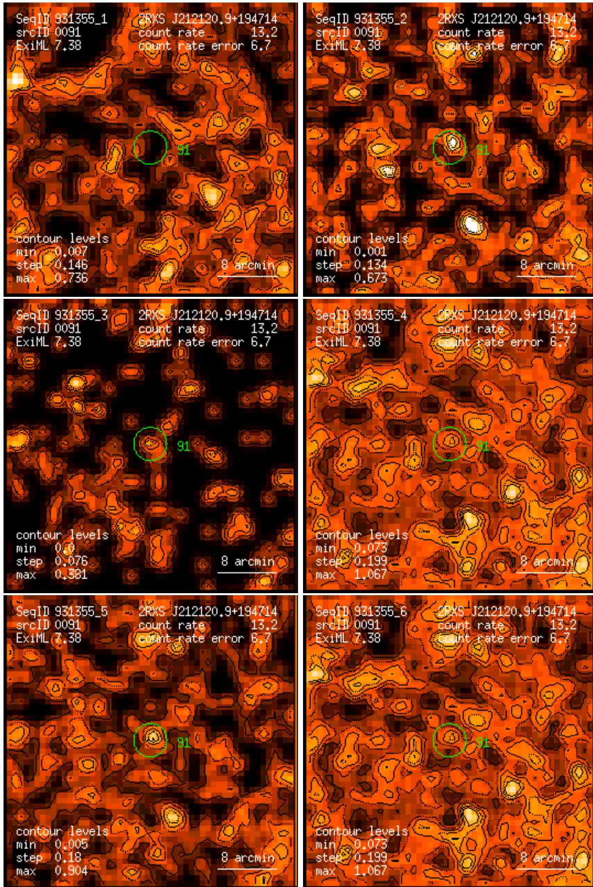
Figure 91: RASS 931355: detection 0091: band rate images, Gaussian filter: (1) PSPP channels 11 – 41, (2) 52 – 90, (3) 91 – 201, (4) 11 – 235, (5) 52 – 201, (6) 11 – 201. Broad band rates in counts/ks. Band rate contour levels in counts/ks/arcmin 2 .
